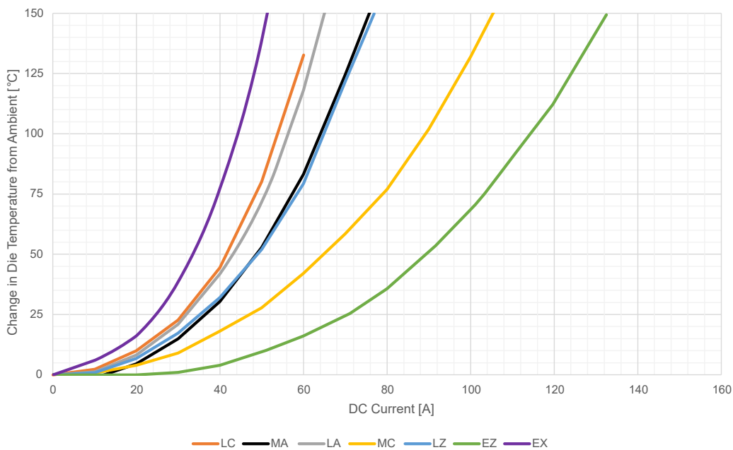
Figure 1: Vias-in-Pad Allegro Lab Results, 25°C
