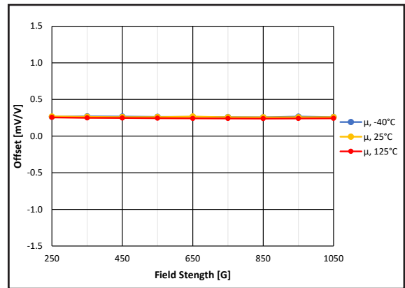
Figure 9: Voltage Offset (mV/V) over Field and Temp
