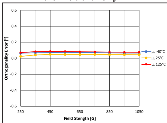
Figure 12: Orthogonality Error over Field and Temp
