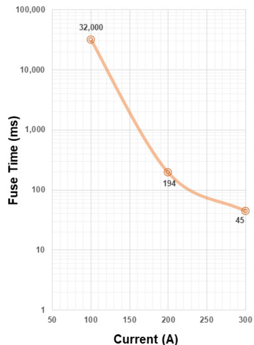
Figure 1: CT43x Fuse Time vs. Current
