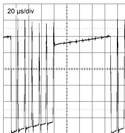
Figure 3. PWM waveform exhibiting seeking behavior
