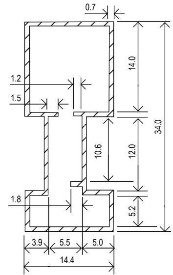
View A-A Enlargement
