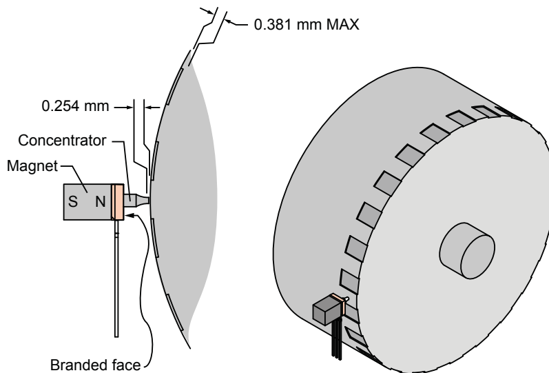
Figure 69. Demonstration of printer drum monitoring application
