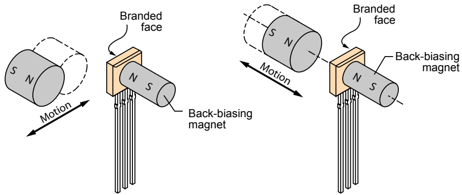
Figure 47. Examples of back-biasing magnet configuration, (left) slide-by and (right) head-on
