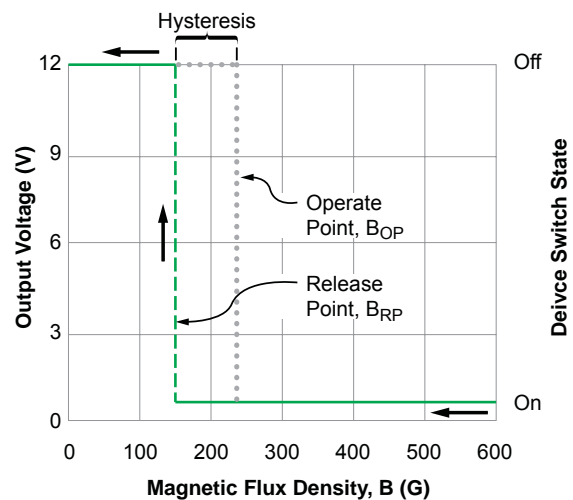
Figure 10. Transfer characteristics of a Hall switch being deactivated (switched off) by the decrease in magnetic flux density from an receding south pole
