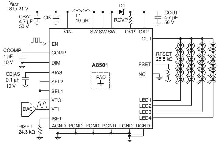
Figure 8. Typical circuit for analog dimming with external DC voltage
