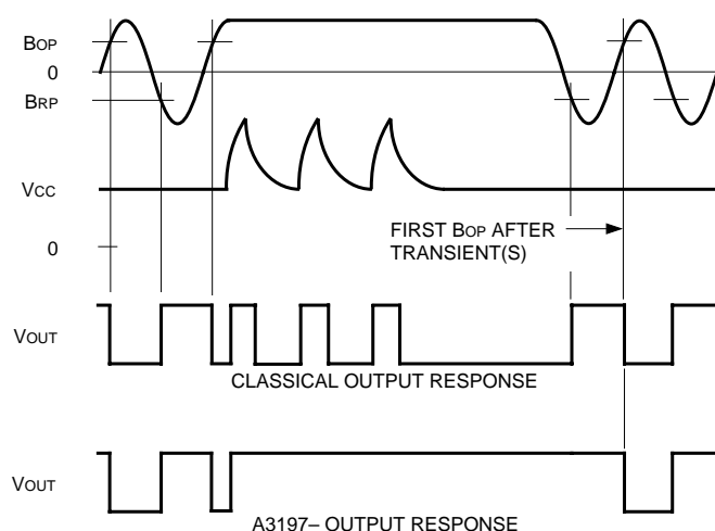
Dwg. WH-007-1A
