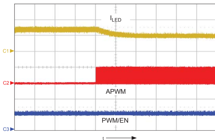
Figure 17. Diagram showing the transition of LED current from 80 mA to 60 mA, when a 25% duty cycle signal is applied to the APWM pin; PWM = 1; shows I_{LED} (ch1, 50 mA/div.), APWM (ch2, 10 V/div.), and PWM/EN (ch3, 5 V/div.), time = 500 \mu s/div.
