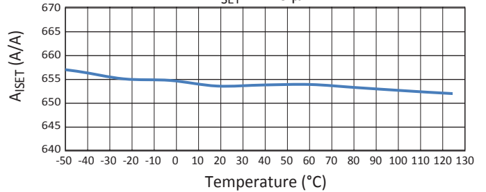
I_{SET} to LED Current Gain versus Ambient Temperature I_{SET} = 120 \mu A
