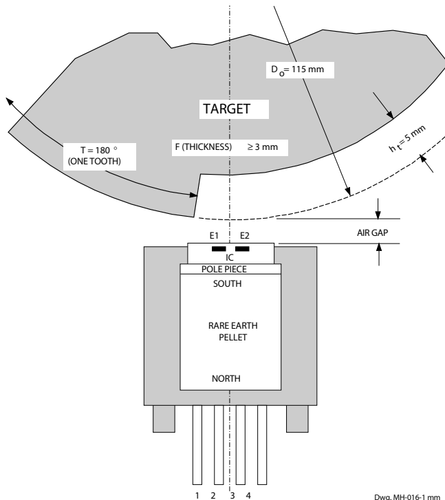
ONE-TOOTH (180°) TARGET
