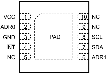
Package EJ, 10-Contact DFN Pinout Diagram
