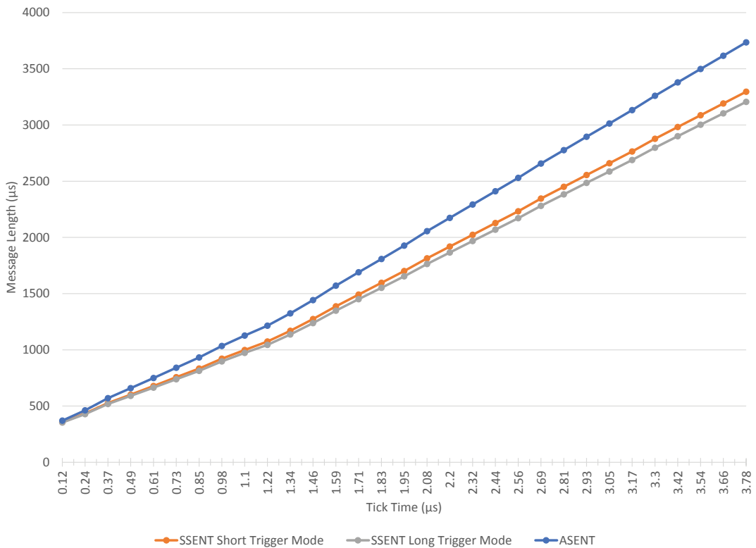
Figure 4: Total Message Length for Four A1346 Sensors with 3 Data Nibbles
