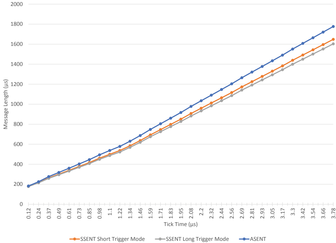
Figure 3: Total Message Length for Two A1346 Sensors with 3 Data Nibbles
