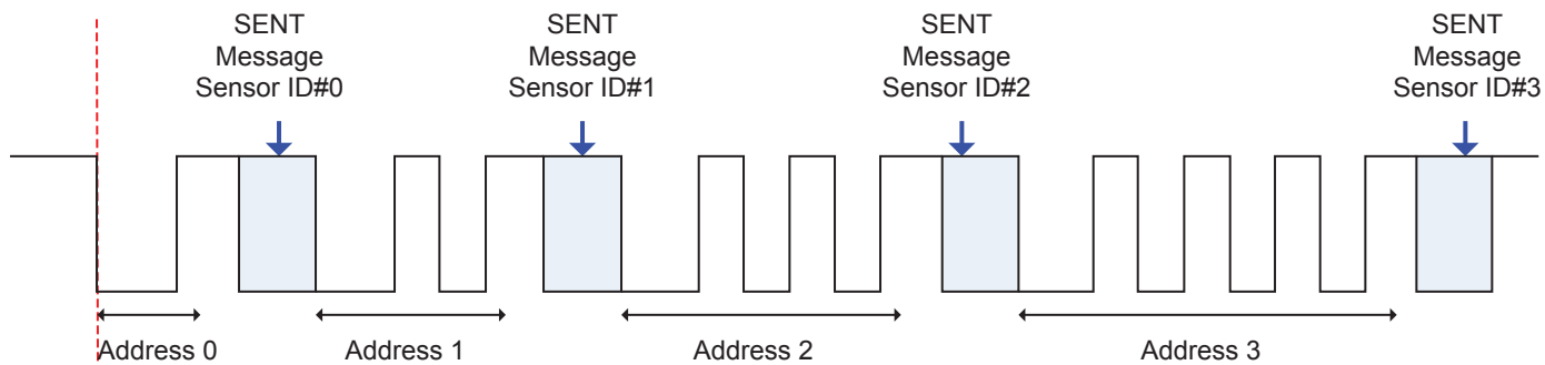
Figure 2: Addressable SENT Output Bus
