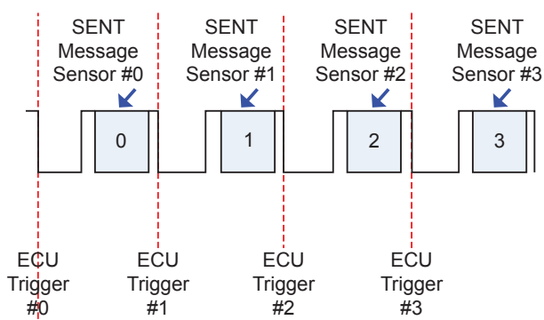
Figure 1: Sequential SENT Output Bus
