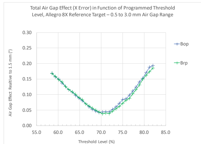
Figure 10: Effect of ATS679PSL threshold change on air gap effect (X error) with Allegro 8X target.
