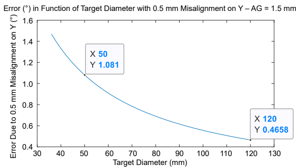
Figure 4: Electrical signal error in function of target diameter, at 0.5 mm of misplacement along Y axis.
