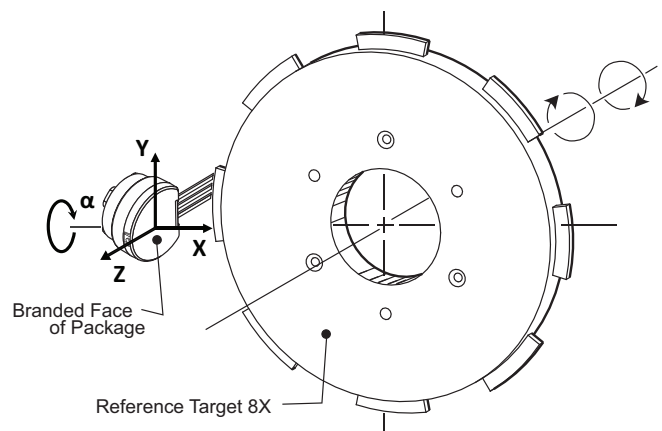
Figure 1: Axes definition for mechanical misalignments on Allegro's ATS679PSL in front of gear tooth target
