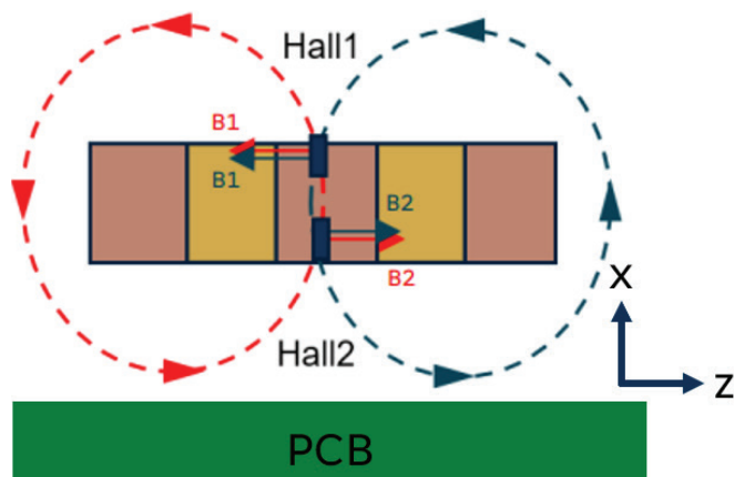
Figure 2: Sensing Concept
