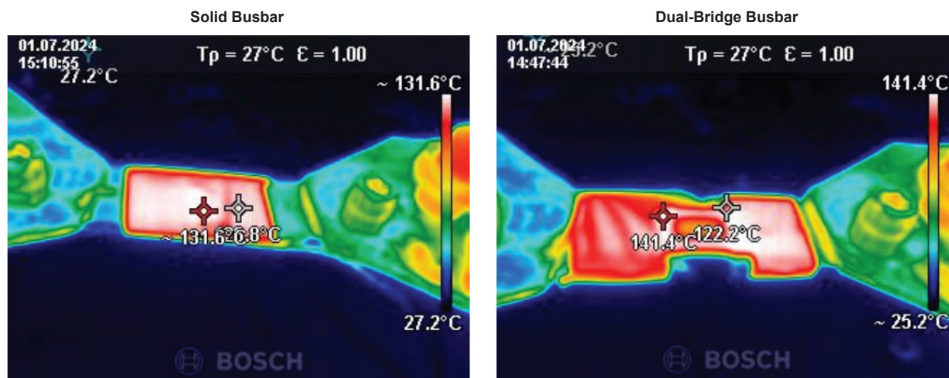
Figure 5: Application of 700 A on 3 mm-Thick Busbars (Cooling System not Used)
