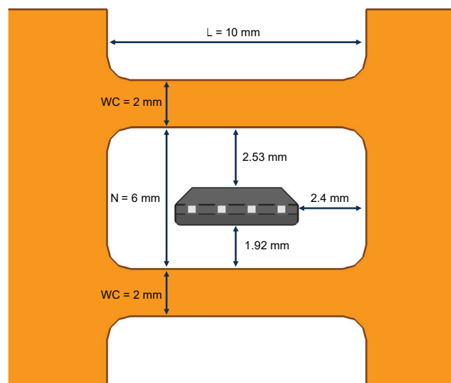
Figure 3: Recommended Design of the Dual Bridge
