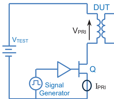
Figure 4: Primary Volt-Second Test Circuit
