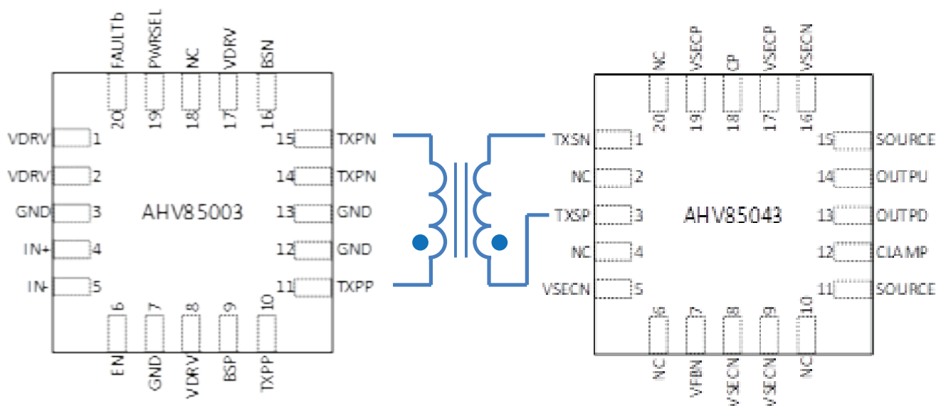
Figure 6: Transformer Interface to AHV85003 and AHV85043
