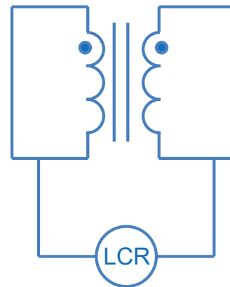
Figure 3: Primary-to-Secondary Capacitance Measurement
