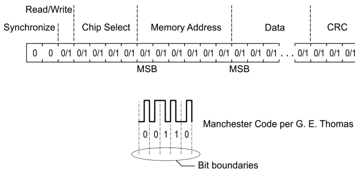
Figure 13: General Format for Serial Interface Commands
