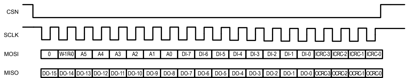
Figure 8: Twenty Bit SPI Transaction
