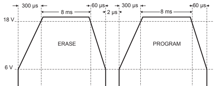
Figure 17: V CC Pulse Profile for EEPROM Programming
