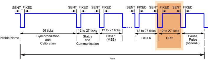
Figure 25: CRC Nibble within the SENT Message Frame
