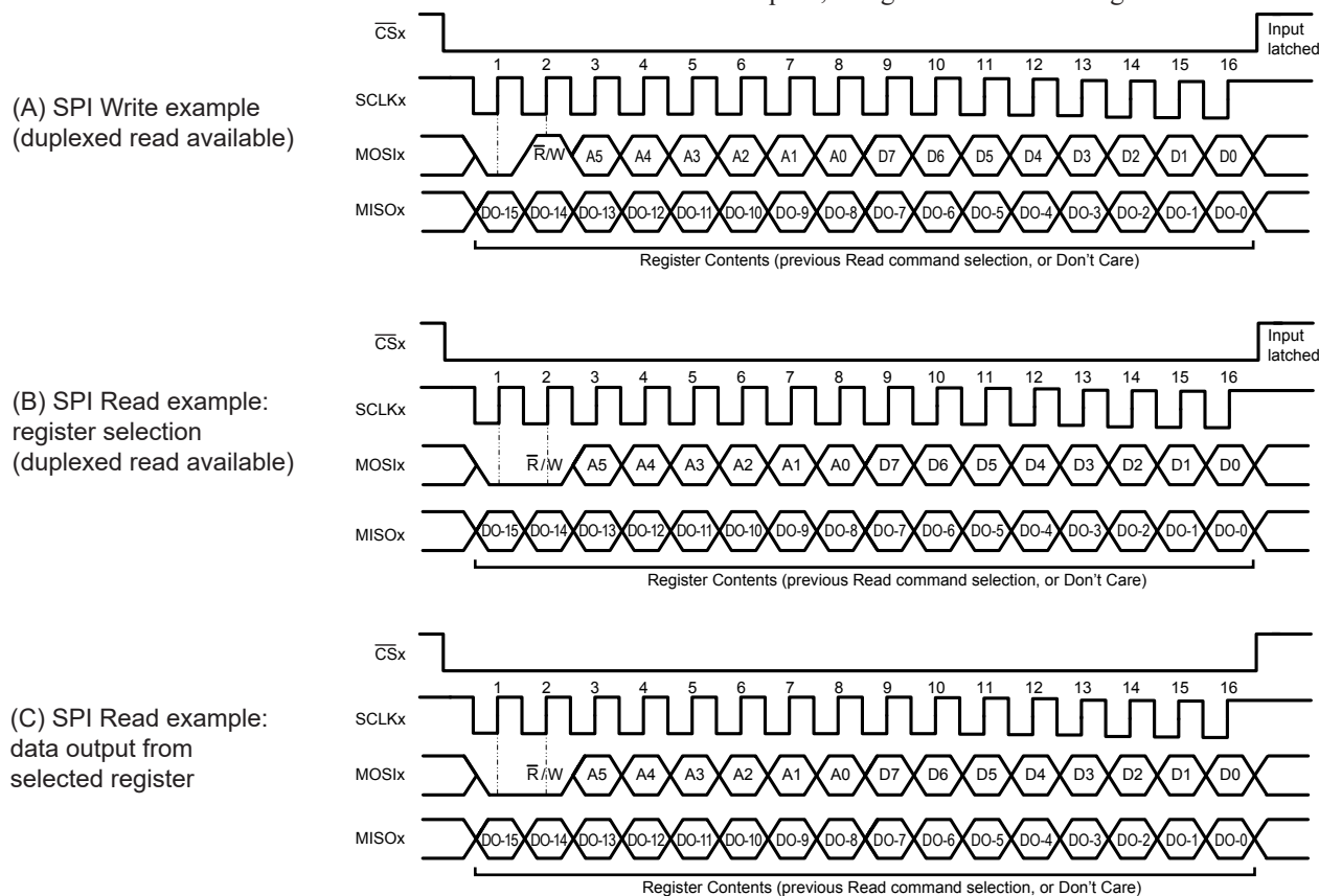
Figure 9: SPI Read and Write Pulse Sequences
