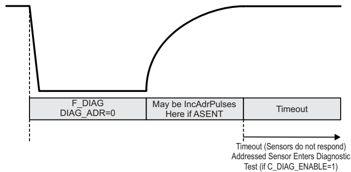
Figure 39: Addressed Diagnostic Request for ASENT and SSENT
