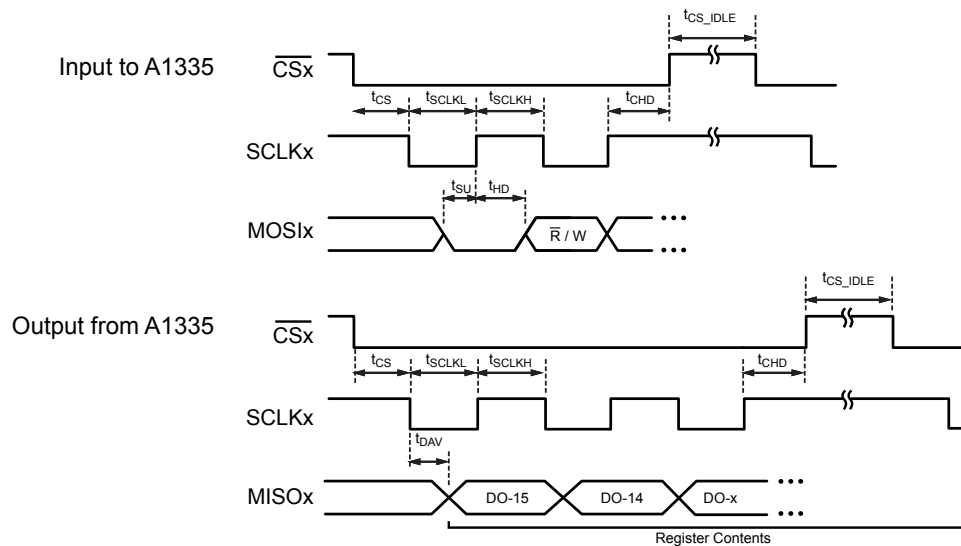
Figure 6: A1335 SPI Interface Timings: (upper) input and (lower) output
