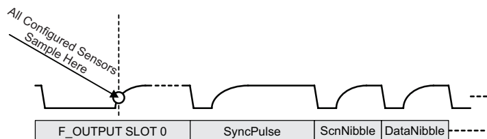
Figure 37: SampleAndHold SSENT with ZERO_SAMPLE = 1
