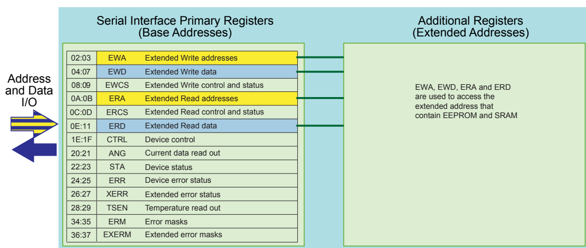
Figure 1: Basic address space for direct access by Serial Interface also provides registers for storing target addresses for extended memory areas, as well as for storing data transferred to and from those areas.
