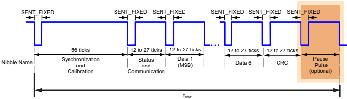
Figure 26: Pause Pulse within the SENT Message Frame
