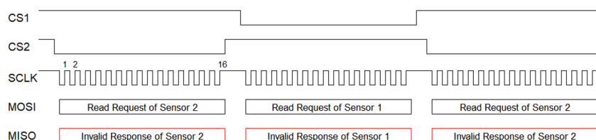
Figure 43: Implementation of SPI using 16-bit packets resulting in IER flag assertion and potentially corrupted data
