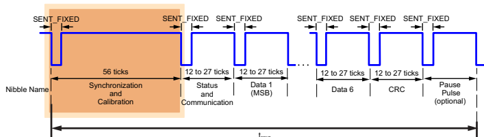
Figure 21: Synchronization and Calibration Pulse within the SENT Message Frame
