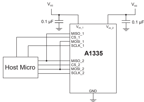
Figure 41: Separate SCLK Lines
