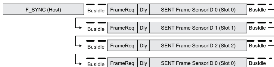
Figure 31: SSENT Sensor Addressing – No Slot Marking (3 Sensors on Bus)
