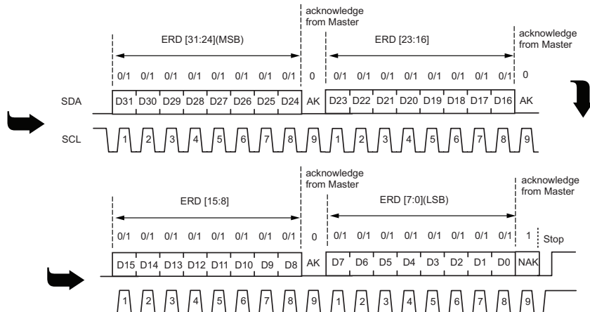
Figure 16: I 2 C Extended Address Read Example
