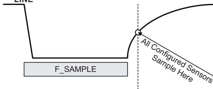
Figure 36: SampleAndHold (SSENT or ASENT)
