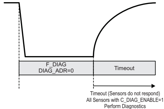
Figure 38: Broadcast Diagnostic Request for ASENT and SSENT
