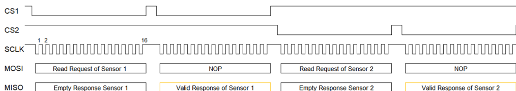
Figure 44: Implementation of SPI using 16-bit packets; valid data, IER flag will still assert
