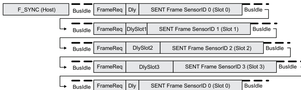
Figure 32: SSENT Sensor Addressing – With Slot Marking (4 Sensors on Bus)
