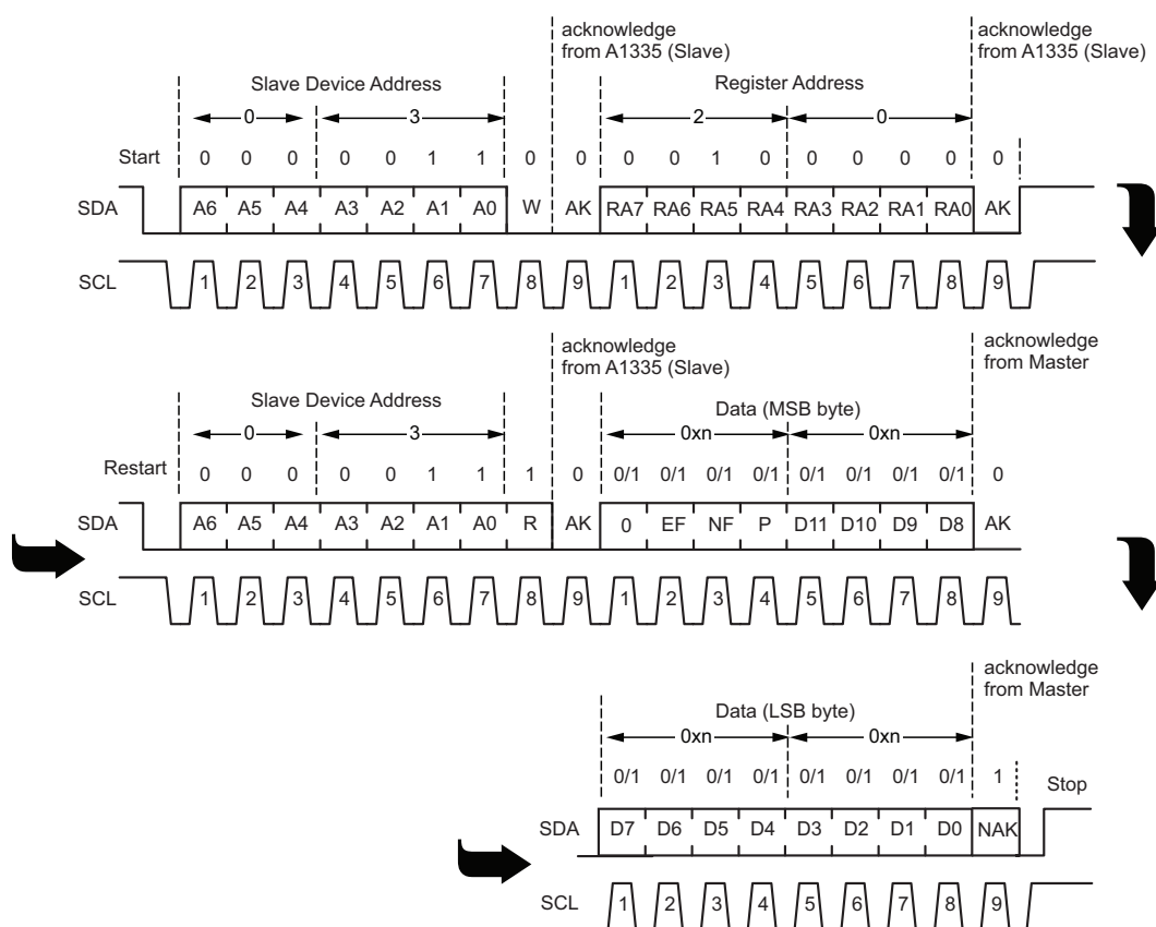
Figure 5: I 2 C Base Address Read: angle value and error status from register address 0x20 (ANG) in slave device 0x3. All steps must occur immediately after the first step, with no intervening transmissions.
