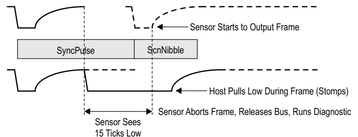
Figure 40: DiagStomp for SENT or TSENT
