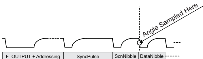
Figure 35: SampleOnOutput Example
