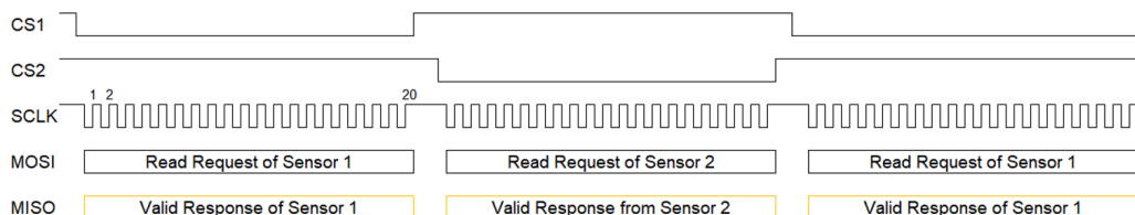
Figure 45: SPI Implementation using 20-bit packets; data contents are valid however IER flag may still assert
