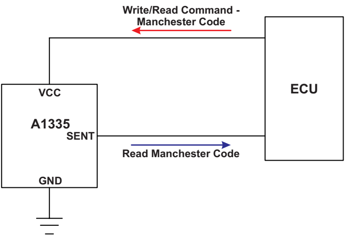
Figure 10: Top-Level Programming Interface
