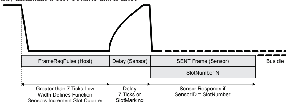
Figure 30: SSENT Sensor Addressing
