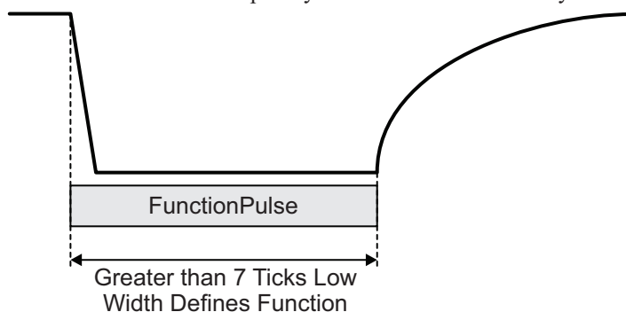
Figure 29: Function Pulse (Output by Host)
