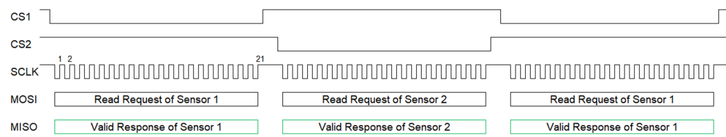
Figure 46: SPI Implementation using 21-bit packets; data contents are valid; no false IER flag generation
