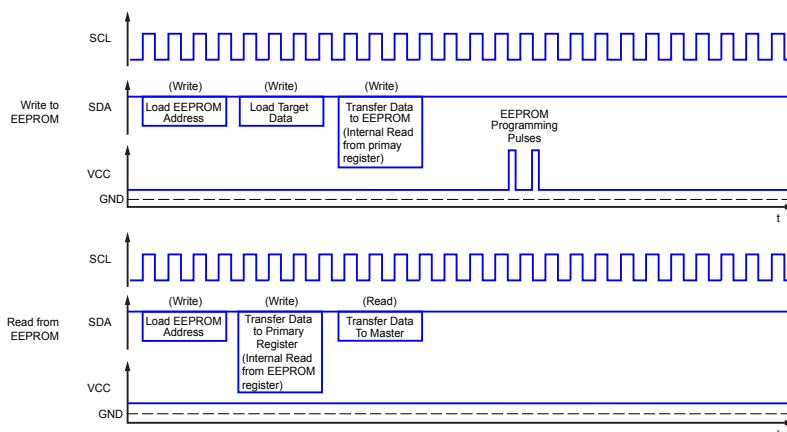
Figure 14: I 2 C Extended Address Write and Read Sessions Examples
