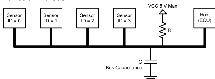
Figure 28: Shared SENT Bus Example
