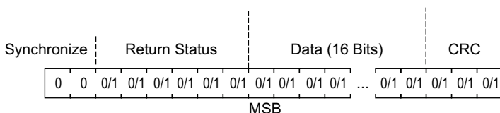
Figure 11: Manchester Read Response
