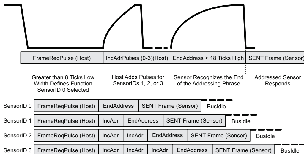
Figure 34: ASENT Sensor Addressing
