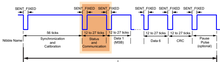
Figure 22: Status and Communication Nibble within the SENT Message Frame
