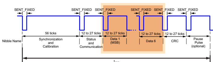
Figure 23: SENT Data Nibbles within the SENT Message Frame
