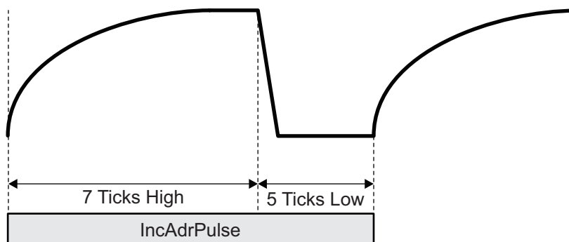
Figure 33: ASENT IncAdrPulse (Output by Host)
