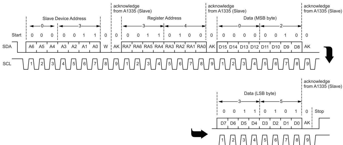
Figure 4: I 2 C Base Address Write: value 0x0235 to register address 0x34 (ERM) in slave device 0x3. All steps must occur immediately after the first step, with no intervening transmissions.
