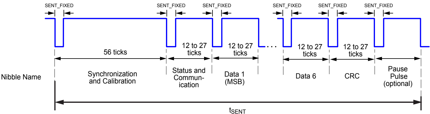
Figure 20: General Format for SENT Message Frame
