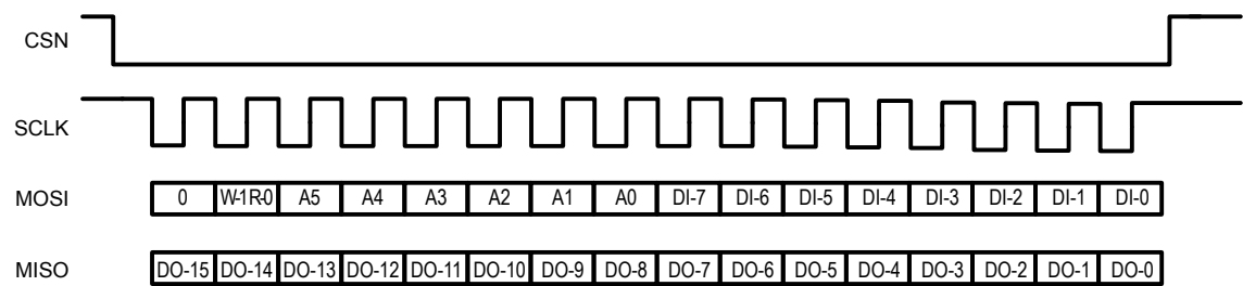
Figure 7: Sixteen Bit SPI Transaction
