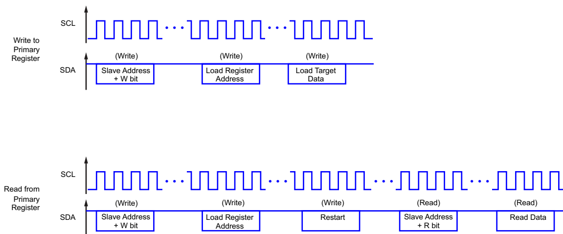
Figure 3: I 2 C Base Address Write and Read Sessions Examples. High-voltage pulses are required on VCC only to invoke an EEPROM write.
