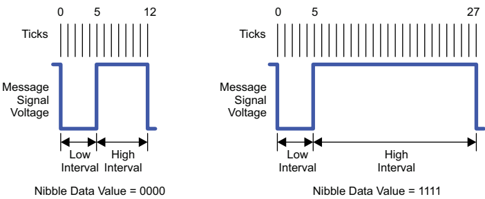
Figure 19: General Value Formation for SENT 0000 (left), 1111 (right)
