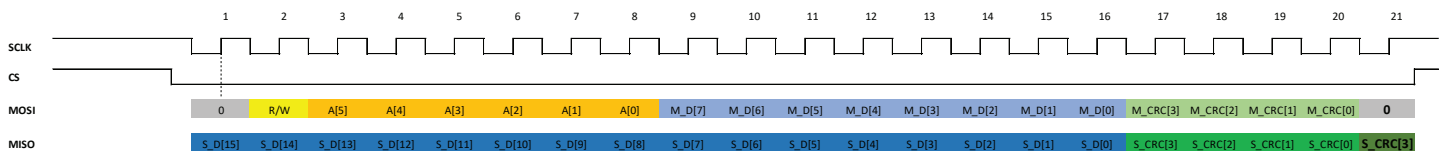
Figure 42: 21-bit SPI Packet Format
