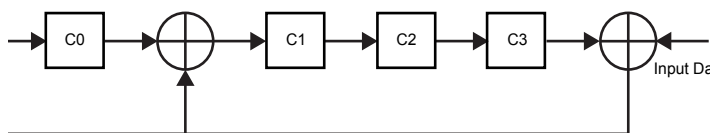
Figure 12: Manchester CRC Calculation
