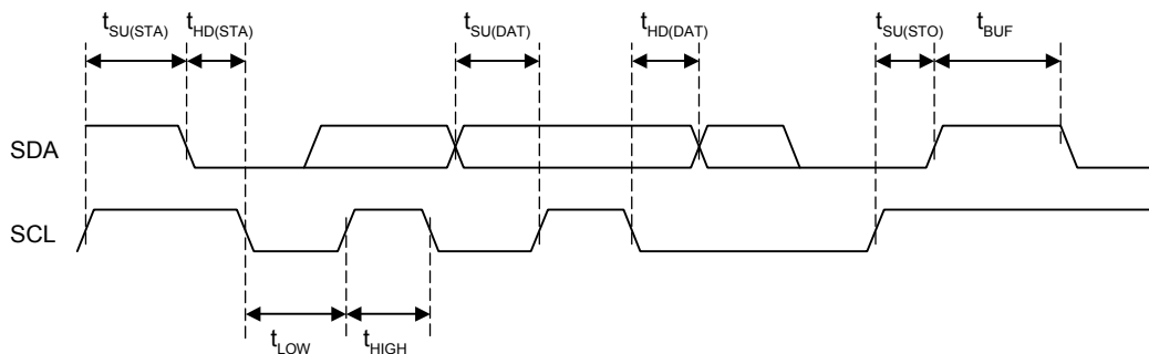
Figure 2: I 2 C input and output timing
