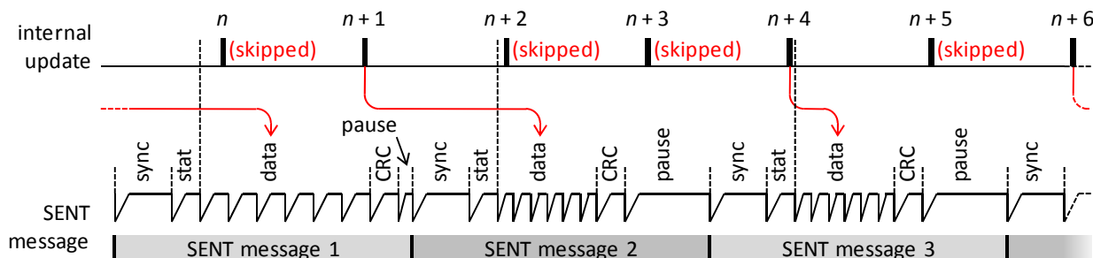
Figure 17: Pause Pulse Used to Extend the Message to Match the Frame Rate ( \text{SENT\_UPDATE} = 1 )
