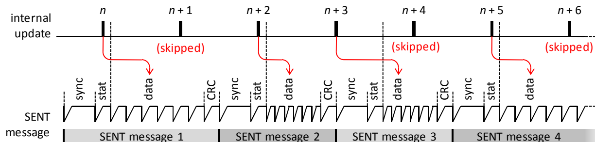
Figure 16: Messages Do not Contain a Pause Pulse ( \text{SENT\_UPDATE} = 0 )
