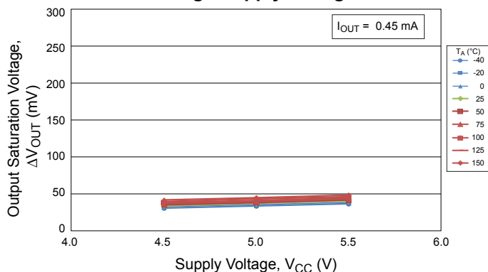
Output Saturation Voltage versus Average Supply Voltage
