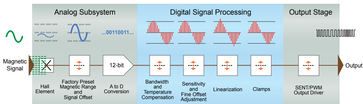
Figure 1: A1341 Signal Processing Path
