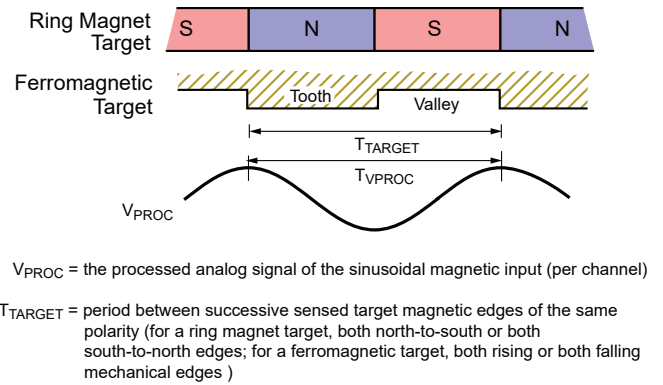
Figure 4: Definition of T_{TARGET}
