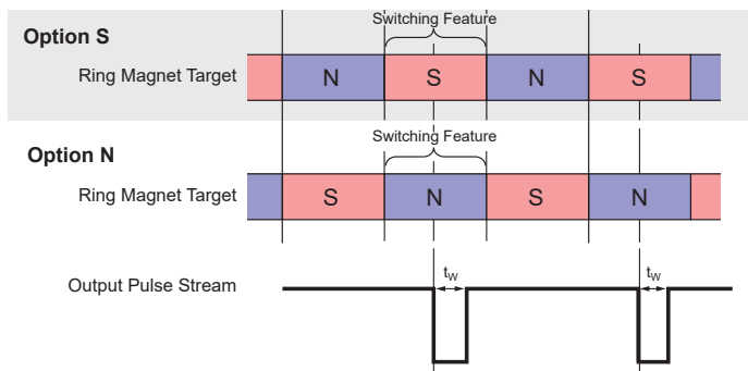
Figure 9: Output Pulse Location
