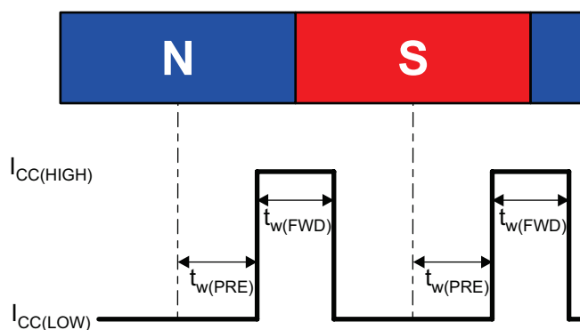
Figure 8: Output Timing Example
