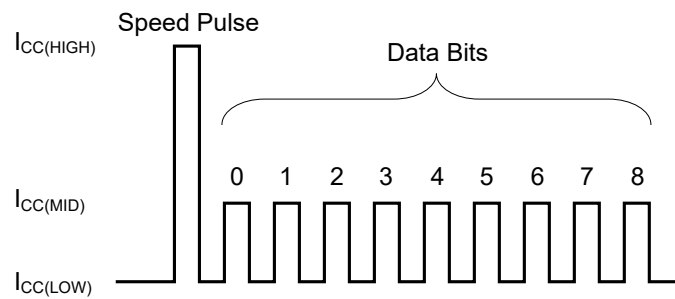
Figure 13: Speed Pulse and Data Bits
