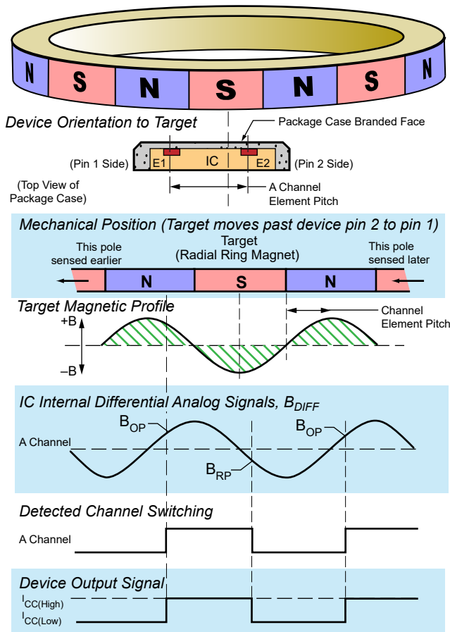
Figure 6: Basic Operation (Ring Magnet)
