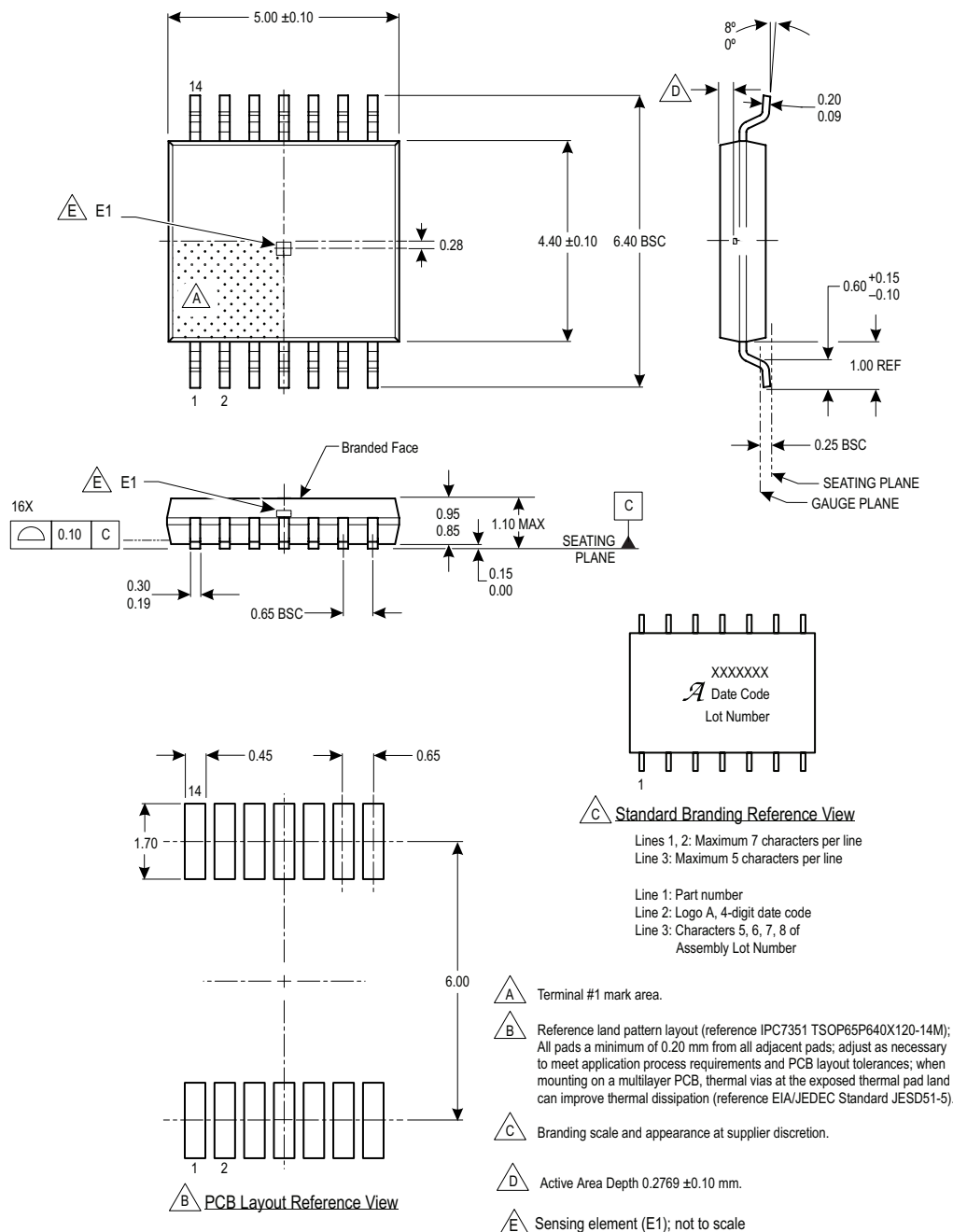
Figure 33: Package LE, 14-Pin TSSOP
