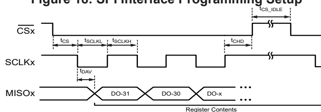
Figure 18: SPI Interface Programming Setup
