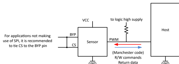
Figure 29: Manchester Programming Interface Setup
