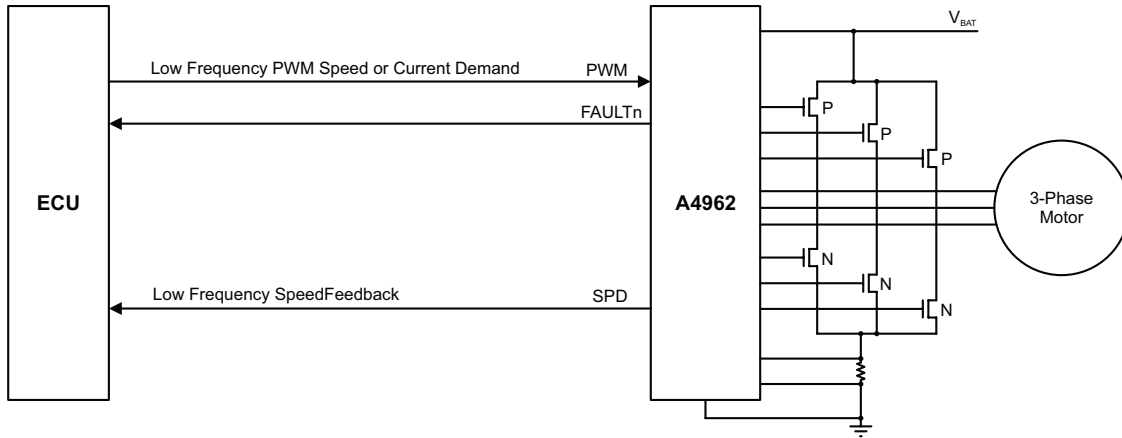
Figure 9: Remote Closed-Loop Control
