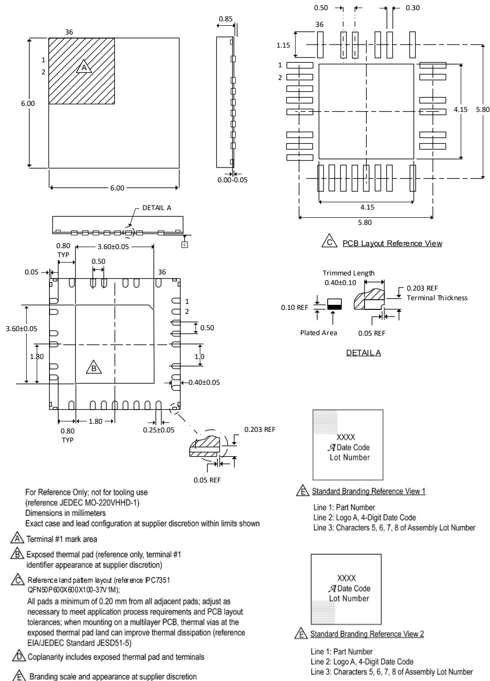
Figure 45: Package EV, 28-Contact QFN with Exposed Pad
