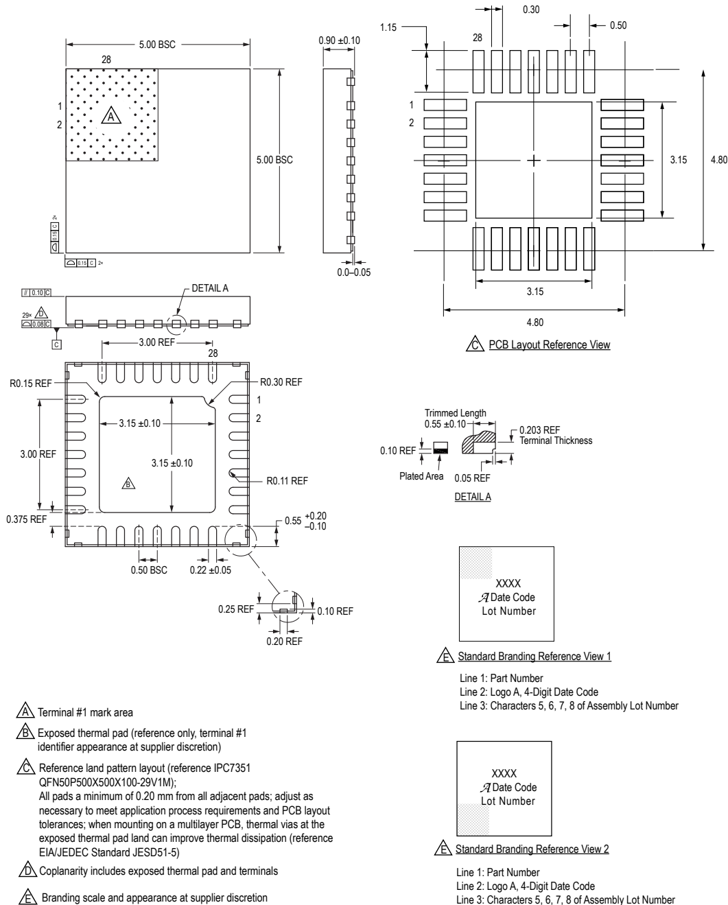
Figure 46: Package ET, 28-Contact QFN with Exposed Pad
