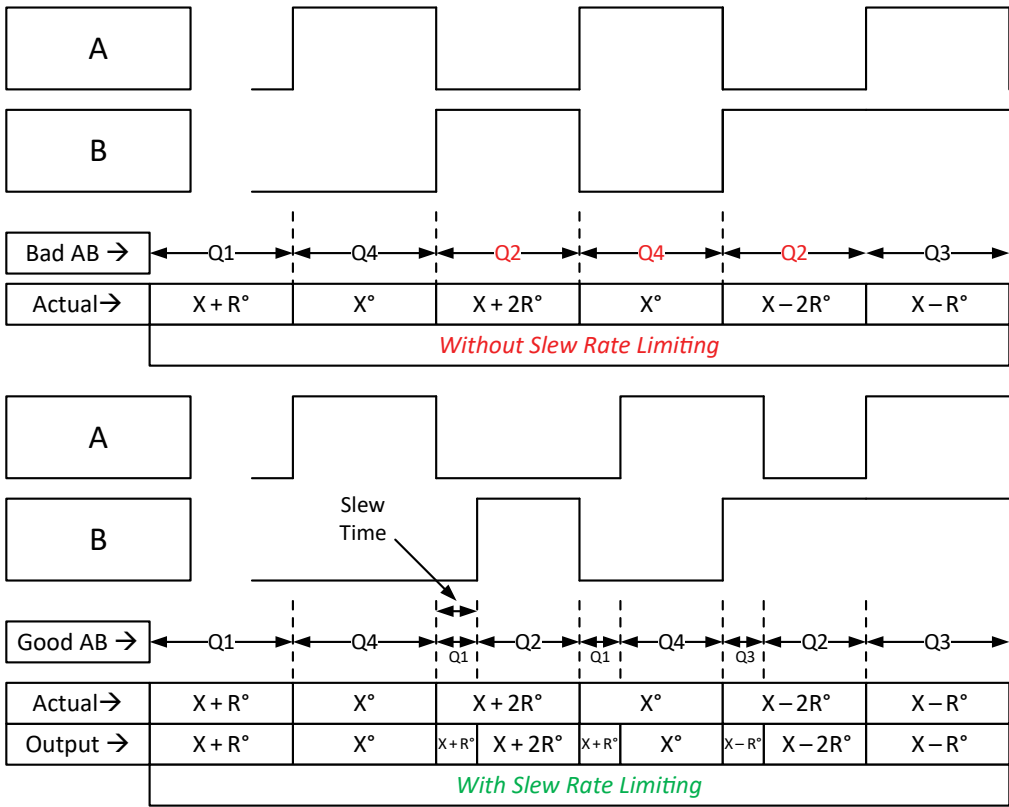
Figure 8: Slew-Rate Limiting
