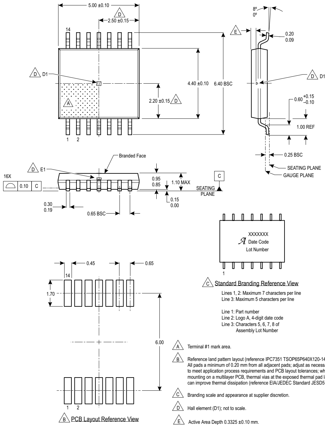
Figure 36: Package LE, 14-Pin TSSOP
