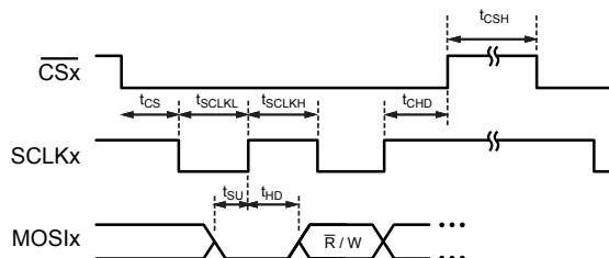
Figure 16: SPI Interface Timing Input
