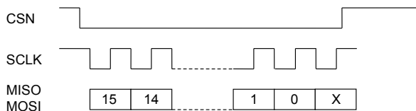
Figure 19: 17-Bit SPI Frame
