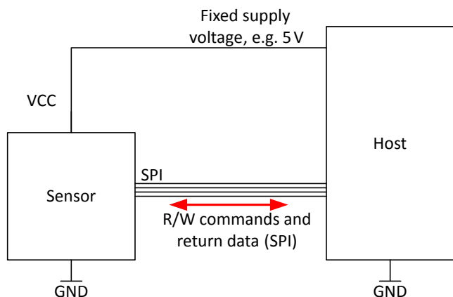
Figure 15: Programming Connections for SPI Interface
