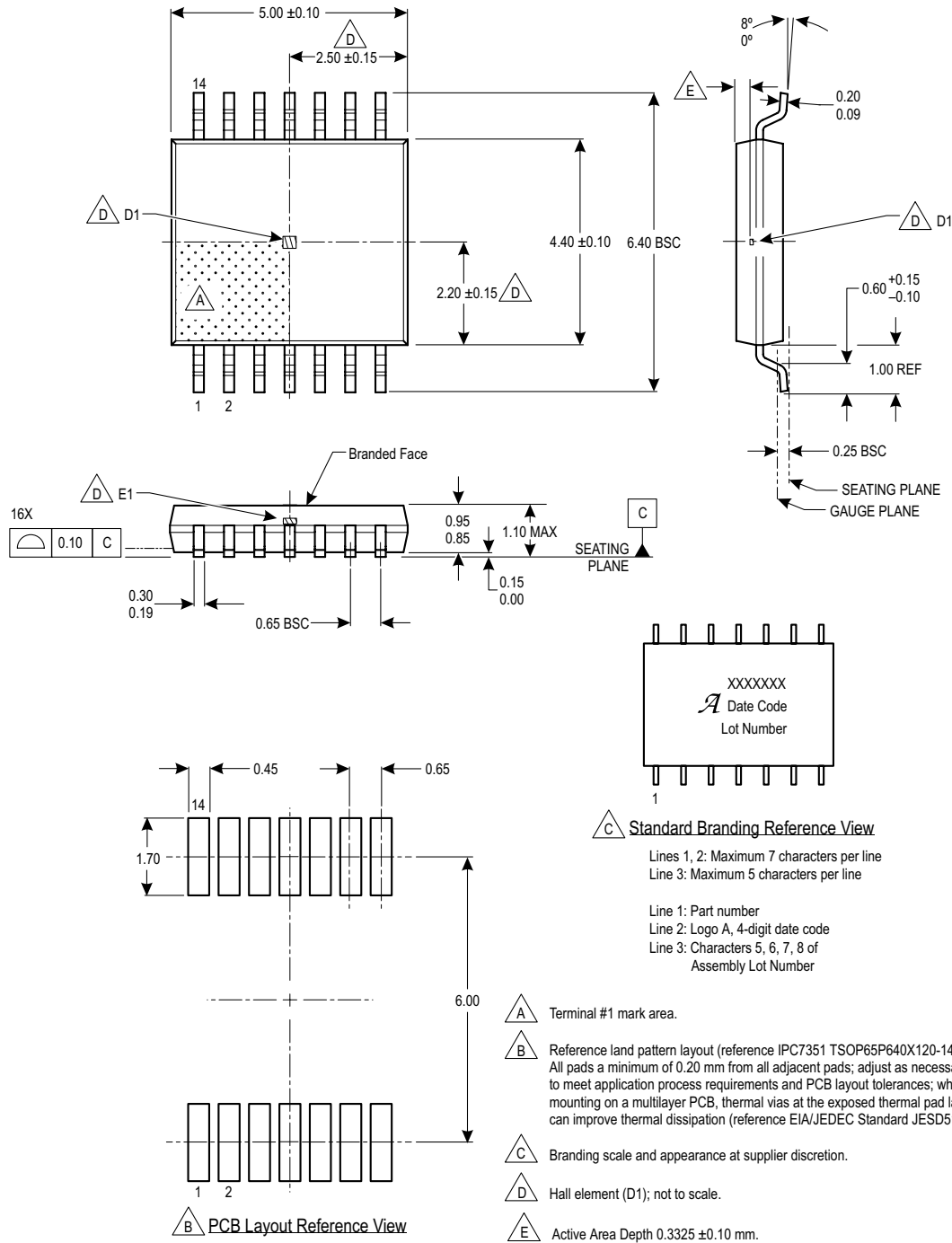
Figure 43: Package LE, 14-Pin TSSOP
