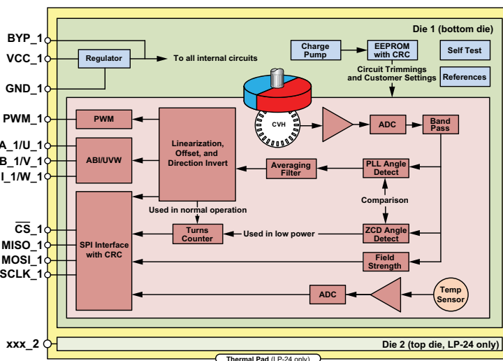
Figure 1: AAS33051 Magnetic Circuit and IC Diagram
