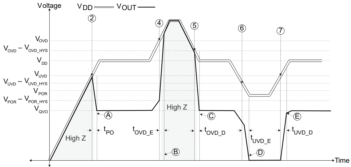
Figure 10: t_{PO} , and t_{OVD}/t_{OVD_R} , and t_{UVD}/t_{UVD_R} with R_{L\_VOUT} = \text{Pull-Up}, 5\text{ V}
