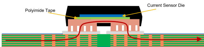
Figure 15: Vias Under Copper Pads (not to scale)
