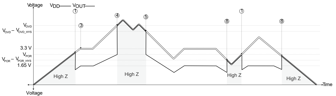
Figure 7: Power States Thresholds with V_{OUT} Behavior, 3.3 V Device, R_L = Pull-Up, UVD Disabled
