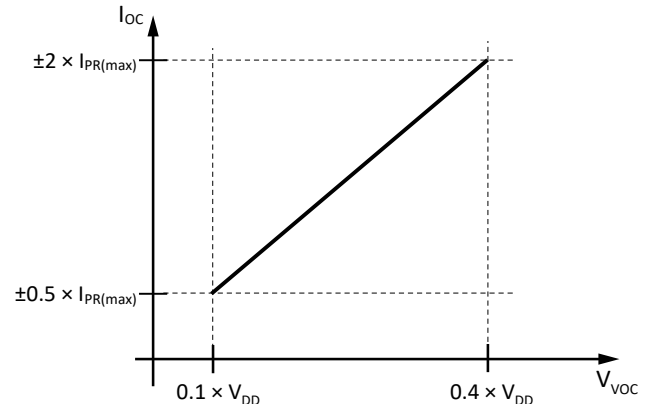
Figure 12: Fault Threshold vs. V_{VOC}
