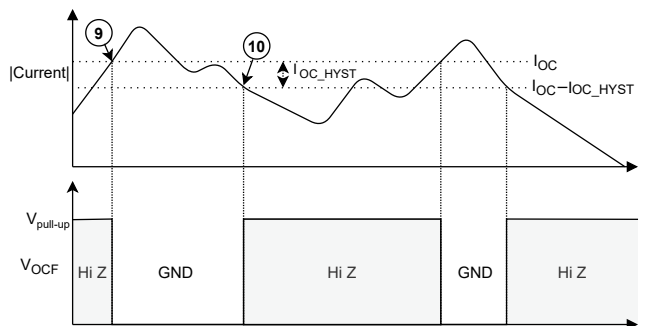
Figure 13: Fault Thresholds and OCF Functionality
