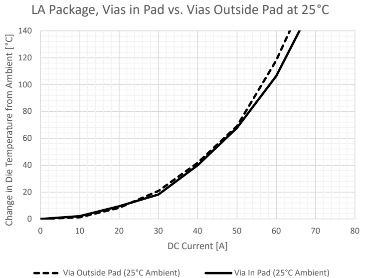
Figure 17: LA Package Performance with/without Vias
