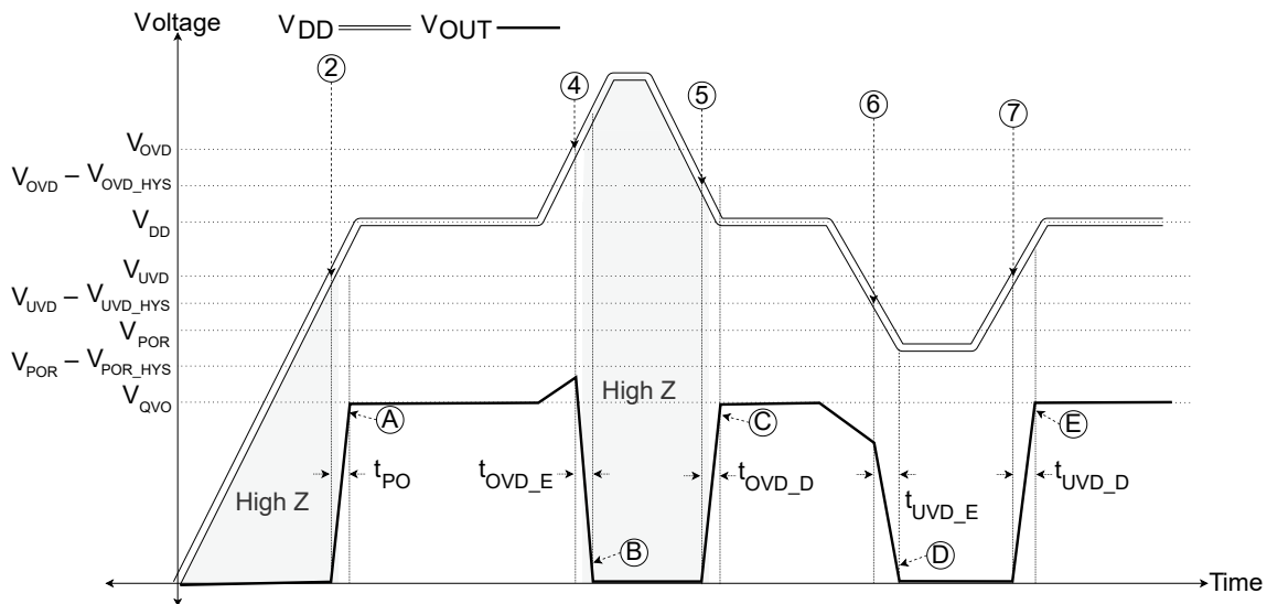
Figure 11: t_{PO} , and t_{OVD}/t_{OVD_R} , and t_{UVD}/t_{UVD_R} with R_{L\_VOUT} = \text{Pull-Down}, 5\text{ V}
