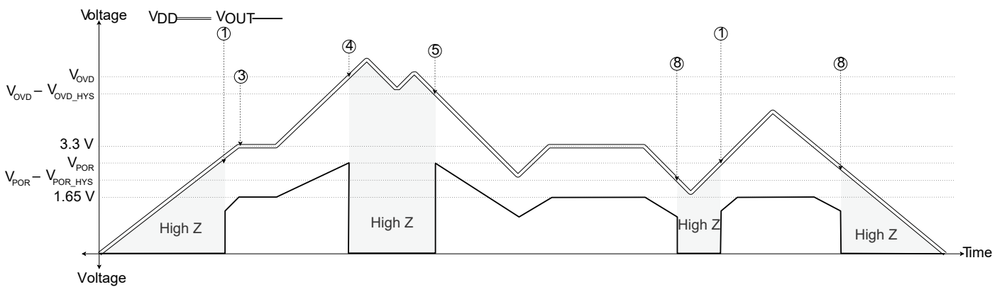
Figure 6: Power States Thresholds with V_{OUT} Behavior, 3.3 V Device, R_L = Pull-Down, UVD Disabled
