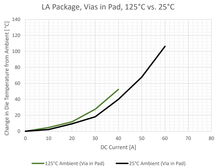
Figure 18: LA Package Performance at 25^\circ\text{C} and 125^\circ\text{C}
