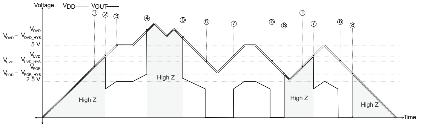
Figure 5: Power States Thresholds with V_{OUT} Behavior, 5 V Device, R_{L\_VOUT} = Pull-Up
