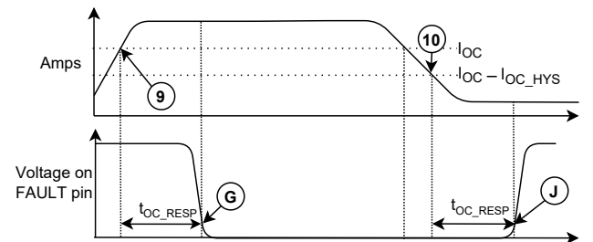
Figure 14: Fault Timing Diagram
