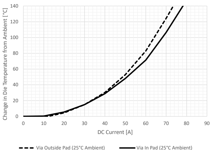
Figure 11: MA Package Performance with/without Vias
