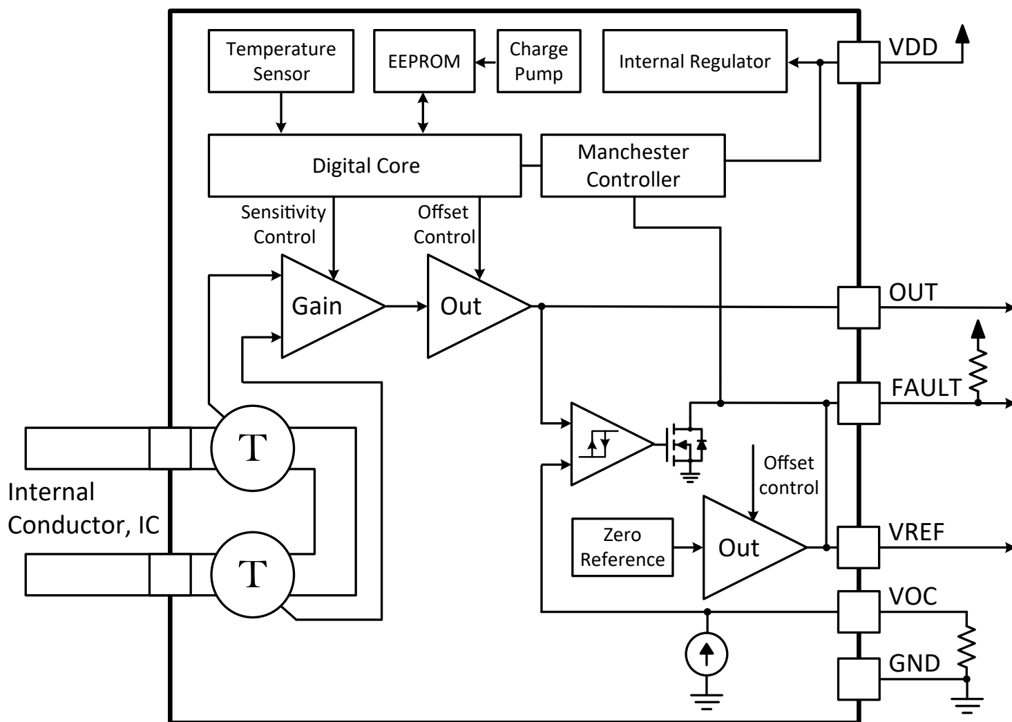
Figure 3: Functional Block Diagram
