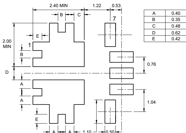
Figure 8: Example Solder Stencil for ACS37220
