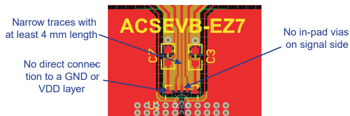
Figure 10: Top Layer of EZ Package Evaluation Board
