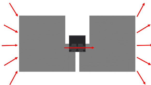
Figure 9: Recommended Trace Layout and Current Flow for IP+ and IP- Pins
