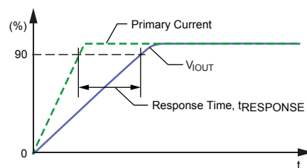
Figure 9: Response Time
