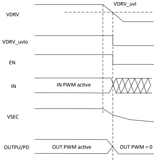
Figure 5: Shutdown Mechanism
