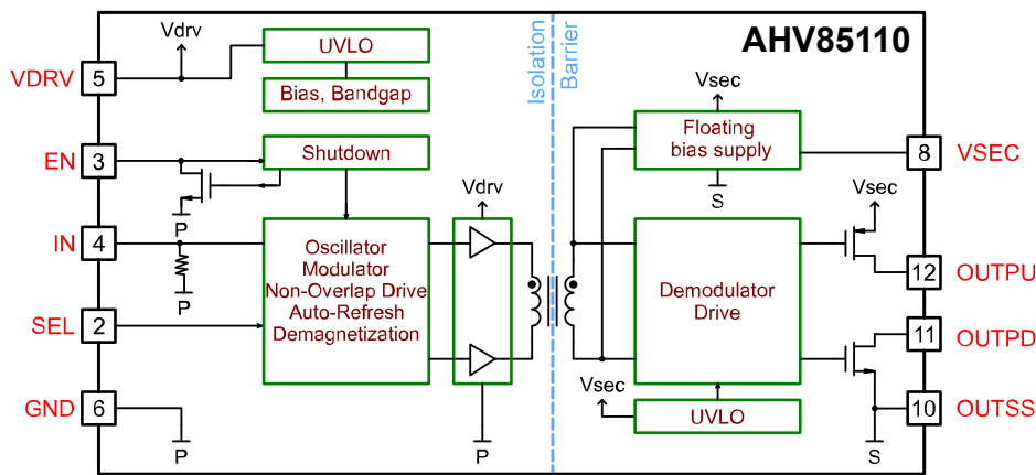
Figure 2: AHV85110 Block Diagram
