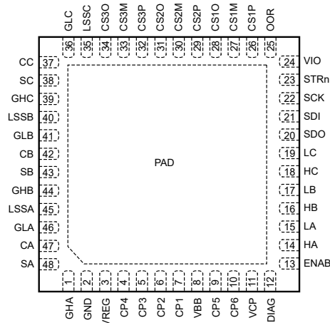
QFN-48 (EV) Package Pinout Diagram
