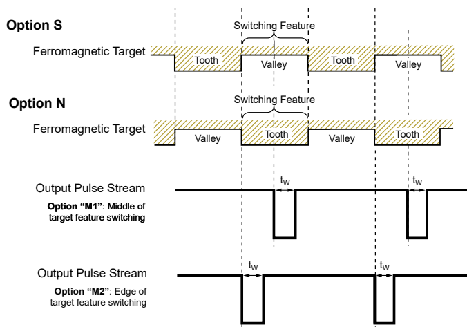
Figure 10: Output Pulse Location (-Wxxxxxxx variant)
