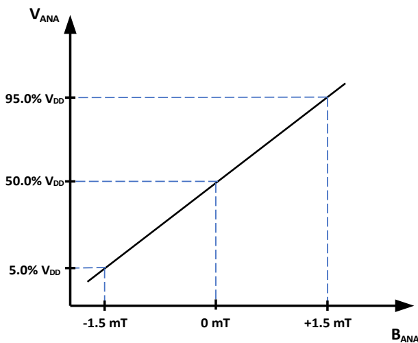
Figure 14: Linear Output Voltage Range vs. Measured Current for G = 300 \text{ mV/V/mT} and current range of +1.5 mT.
