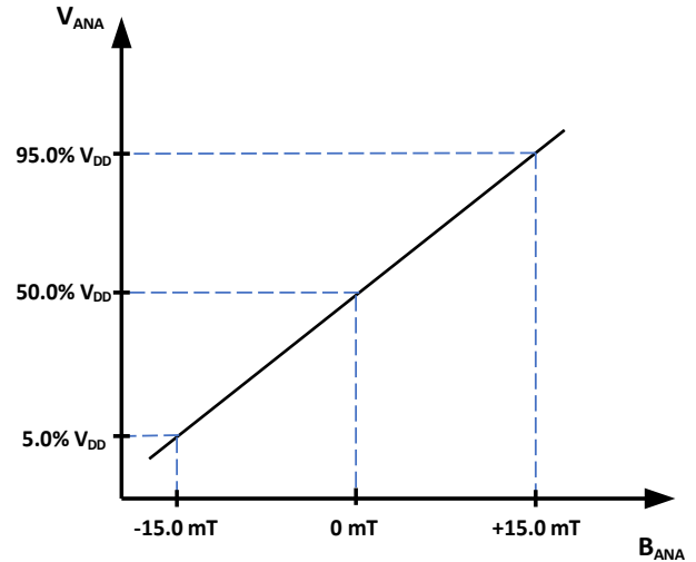
Figure 15: Linear Output Voltage Range vs. Measured Current for G = 30 \text{ mV/V/mT} and current range of +15.0 mT.
