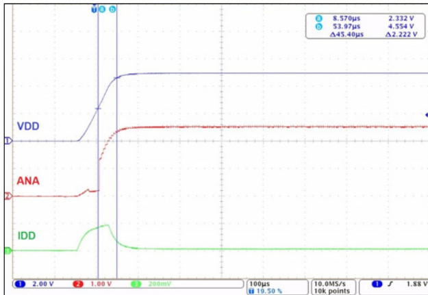
Figure 5: Power-On Time for CT220
