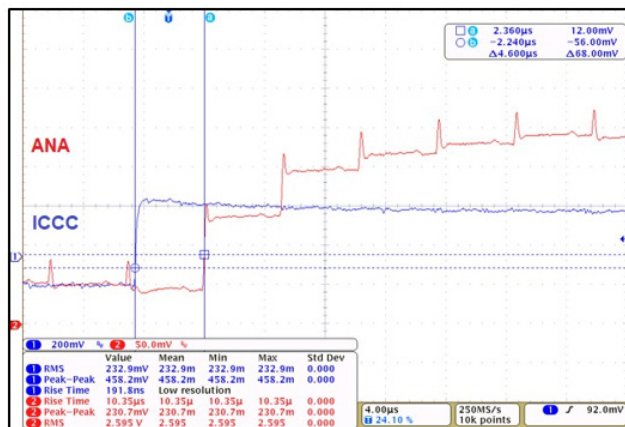
Figure 7: Propagation Delay Time for CT220
