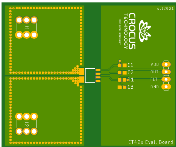
Figure 41: Recommended PCB Layout (Top Layer) for the 20 A to 65 A variants of the CT425
