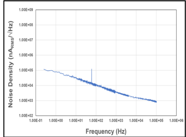
Figure 30: Noise Density vs. Frequency
