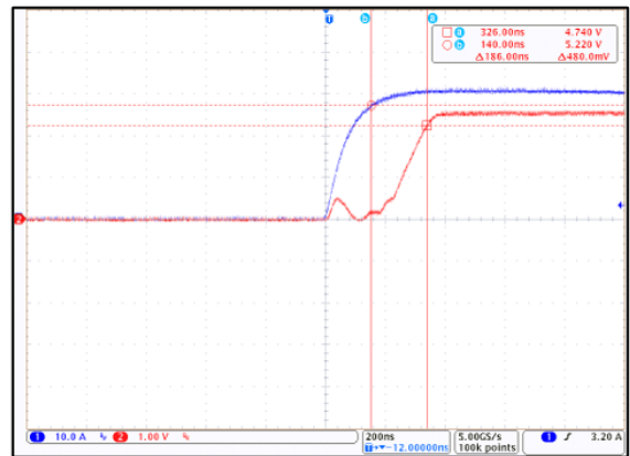
Figure 8: CT425 Response Time; I_P = 30\ \text{A}_{PK} and C_L = 100\ \text{pF} (Blue = I_{CC} , Red = V_{OUT} )
