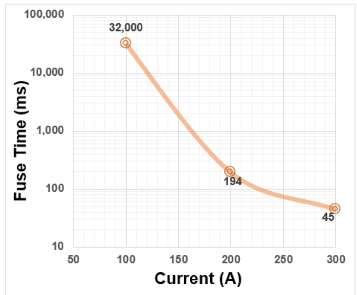
Figure 40: CT432 Fuse Time vs. Current
