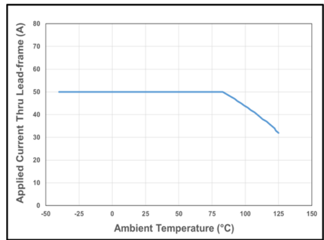
Figure 22: CT432 Current Derating Curve for 50 A DC
