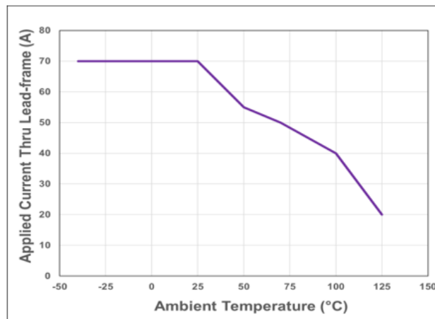
Figure 33: CT432 Current Derating Curve for 70 A RMS
