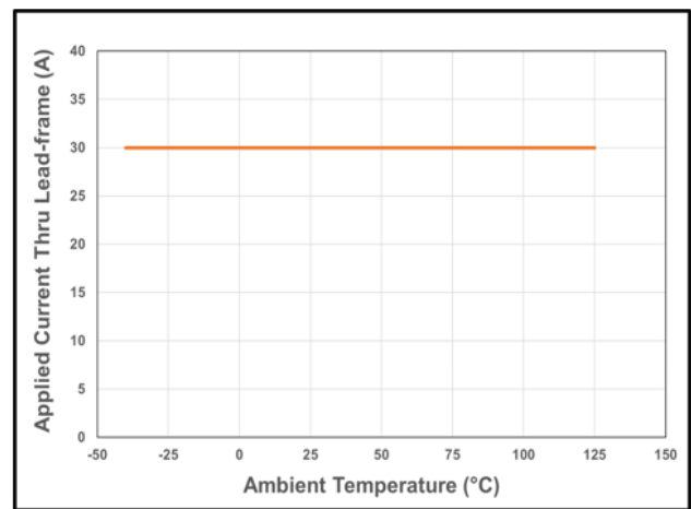
Figure 16: CT432 Current Derating Curve for 30 A DC
