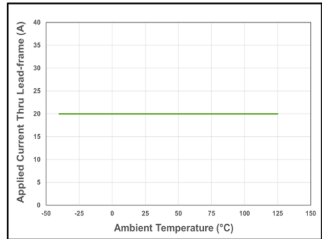
Figure 10: CT432 Current Derating Curve for 20 A DC
