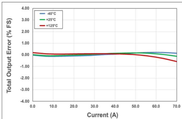
Figure 32: Total Output Error vs. Current vs. Temperature
