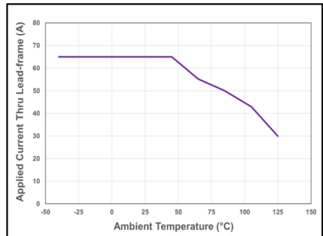
Figure 28: CT432 Current Derating Curve for 65 A DC
