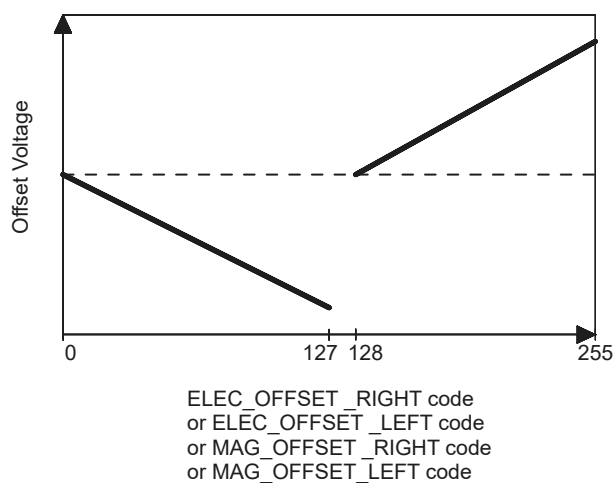
Figure 10: Offset voltage behavior with ...OFFSET... codes variations
