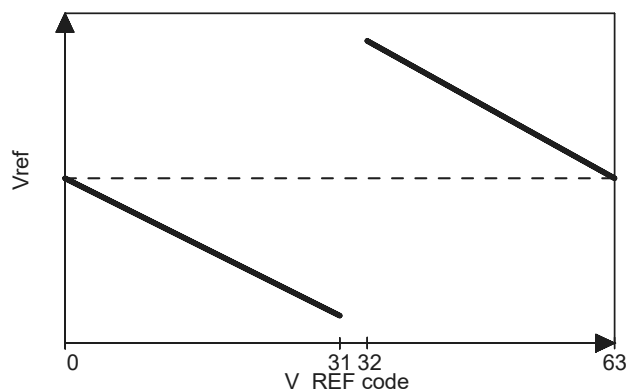
Figure 8: Vref behavior with V_REF code variations
