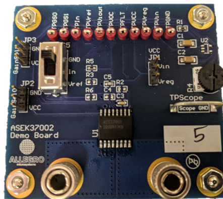
Figure 1: ASEK37002 Evaluation Board
