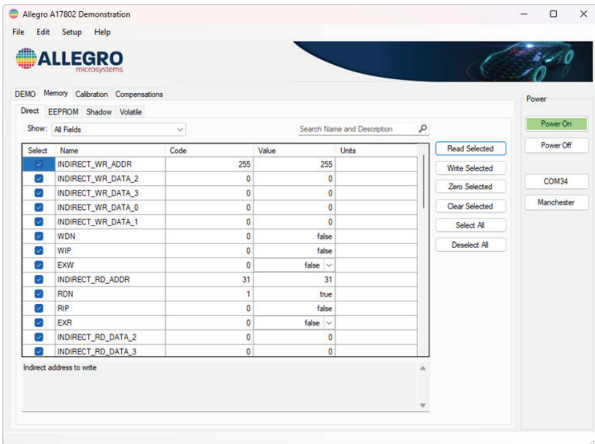
Figure 7: Memory Tab
