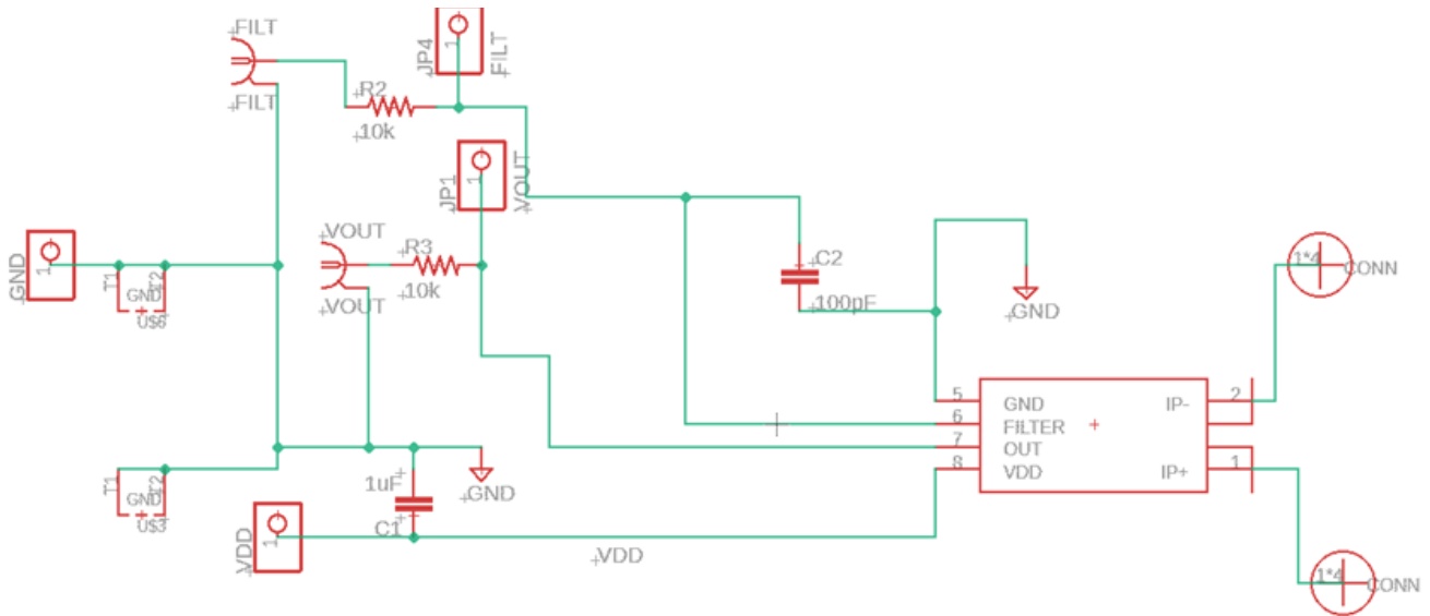
Figure 3: CT416-50AC Evaluation Board Schematic
