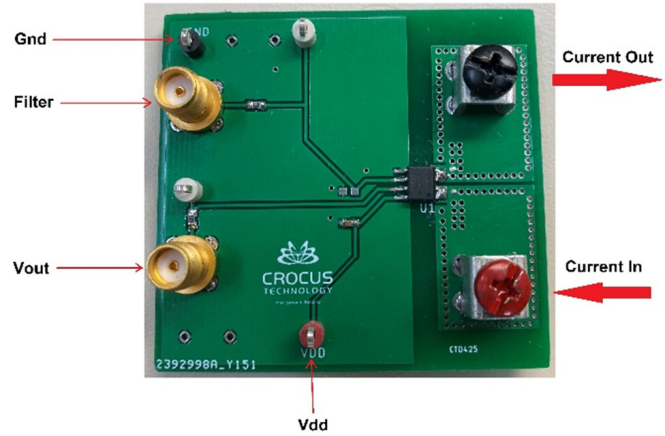
Figure 1: CT416-50AC Evaluation Board
