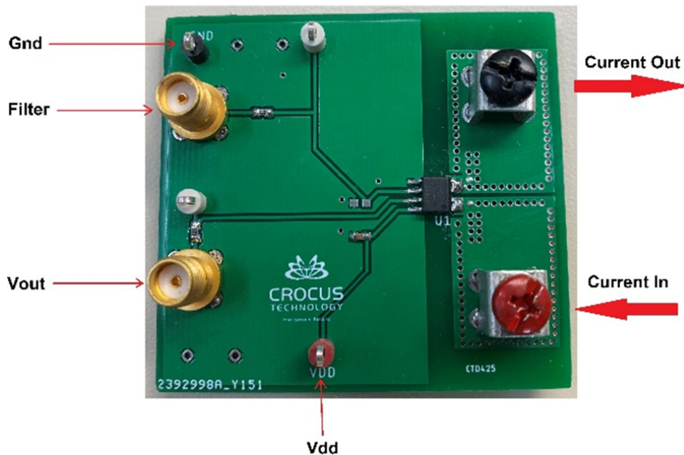
Figure 2: CT416-50AC Evaluation Board
