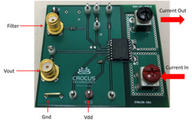
Figure 1: CT433-50AC Evaluation Board
