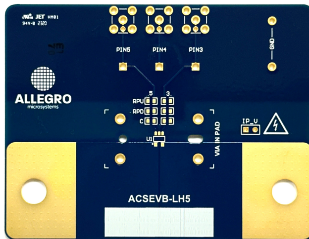
Figure 1: LH Bare Evaluation Board
