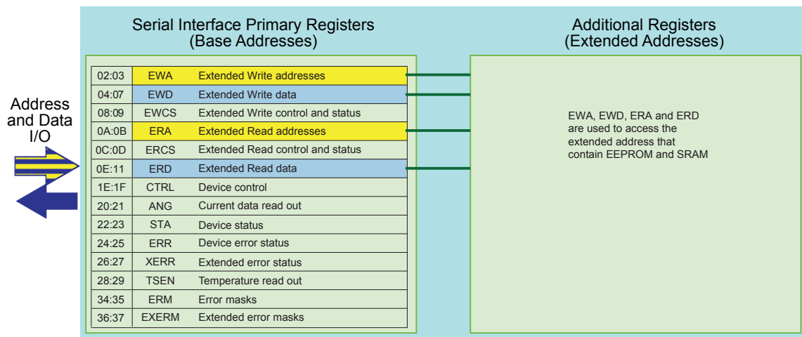
Figure 1: Basic address space for direct access by Serial Interface also provides registers for storing target addresses for extended memory areas, as well as for staging data transferred to and from those areas.
