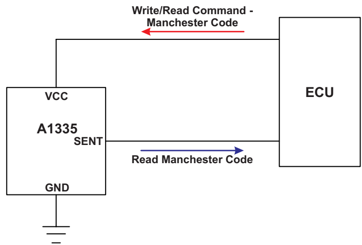
Figure 10: Top-Level Programming Interface
