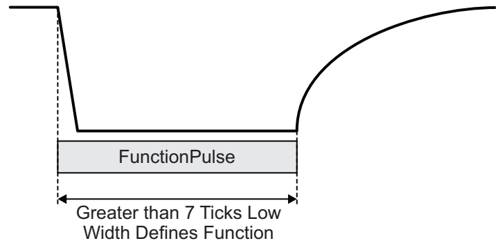
Figure 29: Function Pulse (Output by Host)
