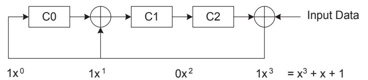
Figure 12: Manchester CRC Calculation
