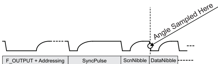
Figure 35: SampleOnOutput Example
