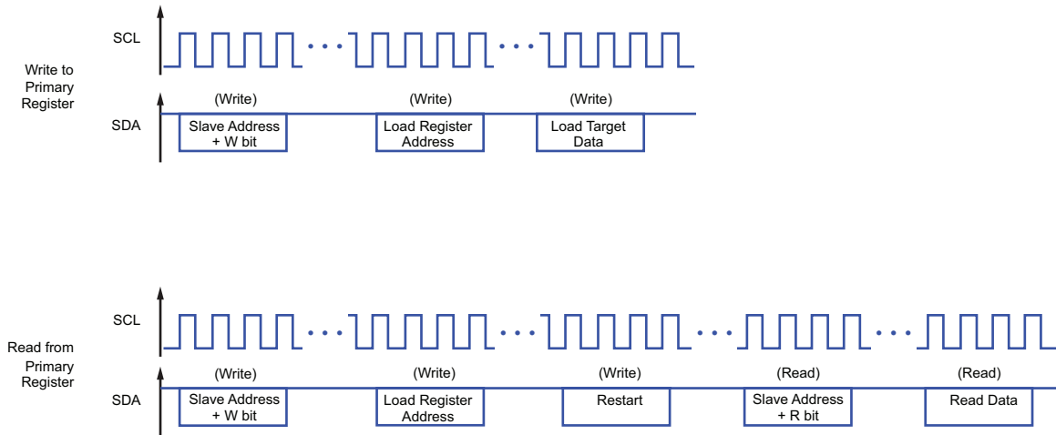
Figure 3: I 2 C Base Address Write and Read Sessions Examples. High-voltage pulses are required on VCC only to invoke an EEPROM write.
