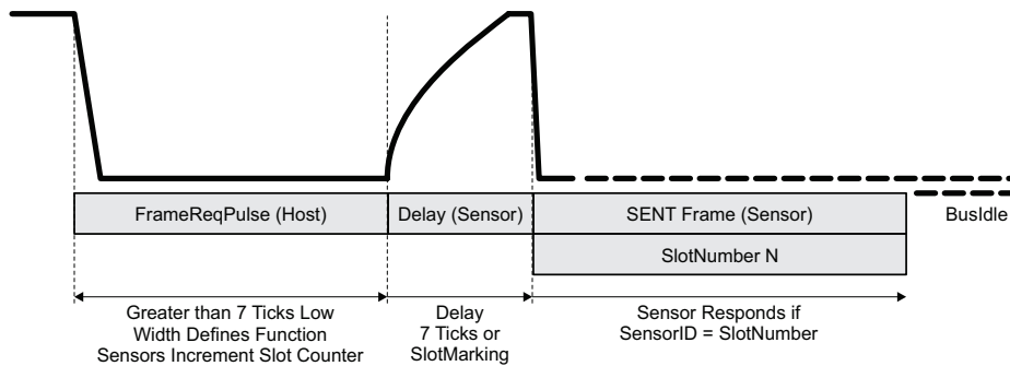
Figure 30: SSENT Sensor Addressing
