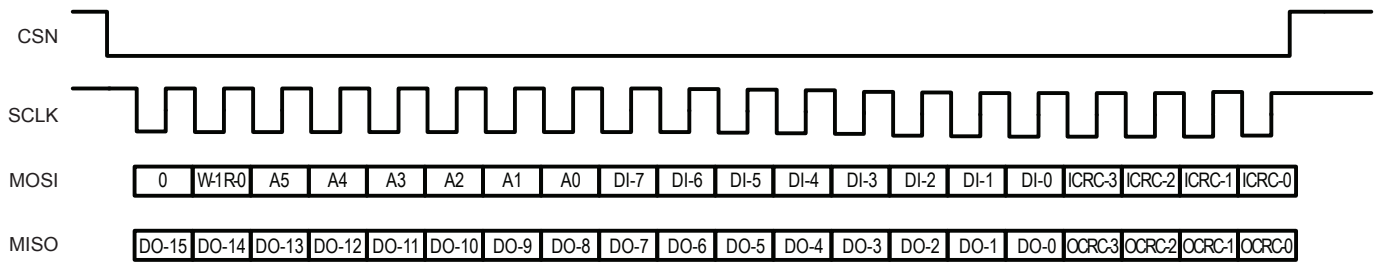
Figure 8: Twenty Bit SPI Transaction
