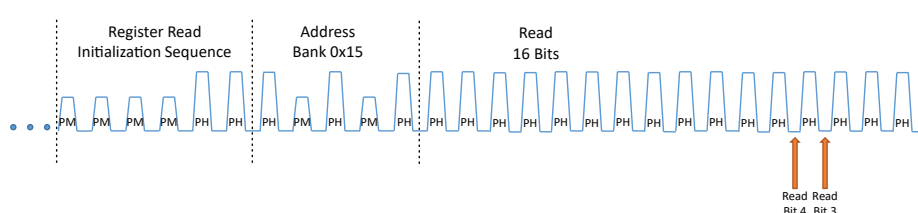
Figure 23: Checking EEPROM Margining Results Pulse Sequence
