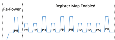
Figure 7: VCC Pulse Sequence to enable Shadow Registers
