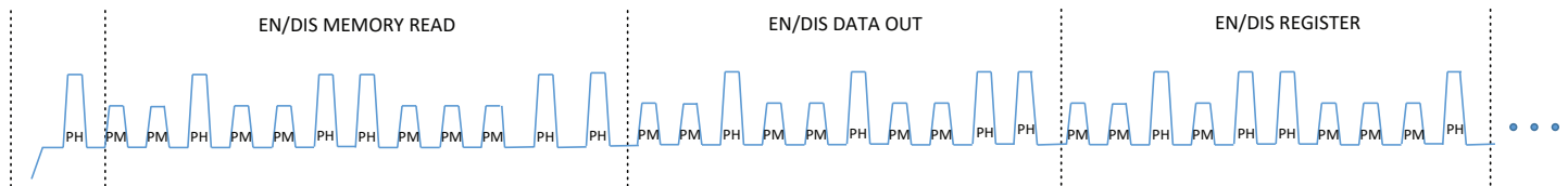
Figure 4: VCC Pulse Sequence to enter Volatile Shadow Registers Readback Mode
