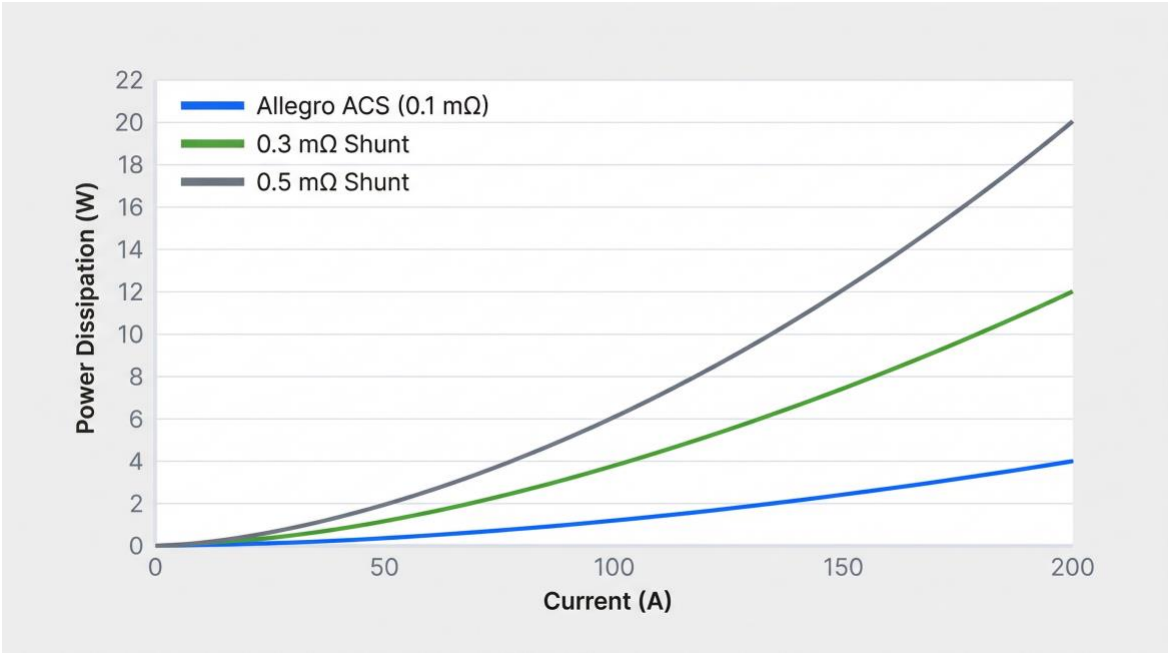
Figure 2. Current vs. power dissipation for shunt and Allegro fully integrated current sensor IC package
