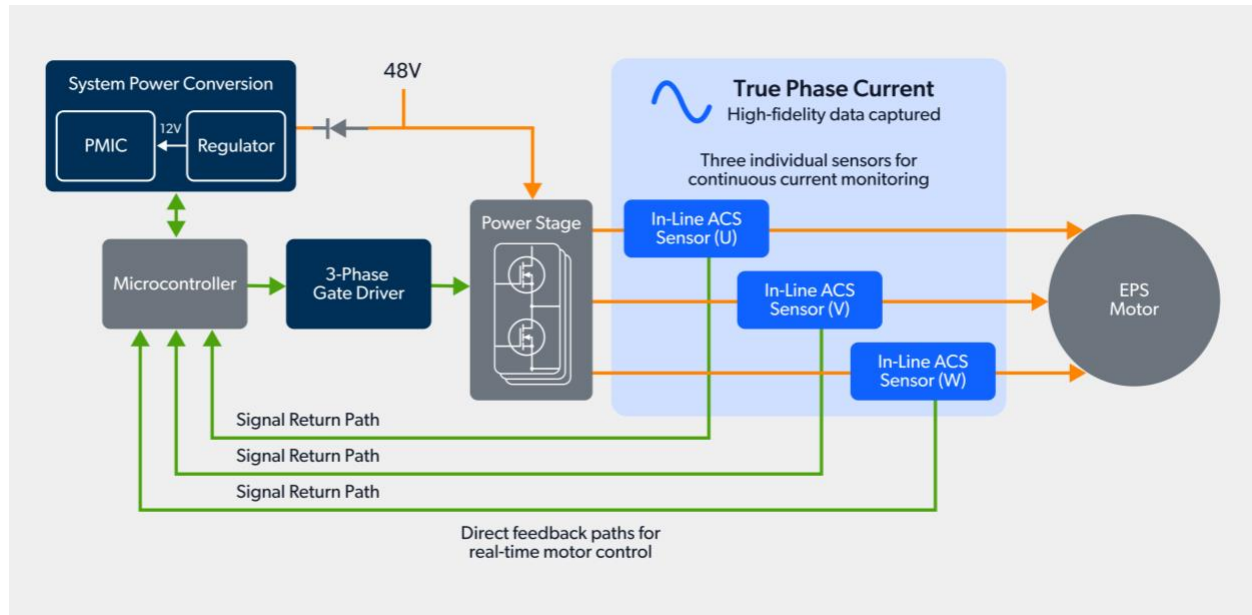
Figure 1. In-Line current sensing architecture for 48V EPS systems
