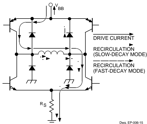
Figure 1 — Load-Current Paths
