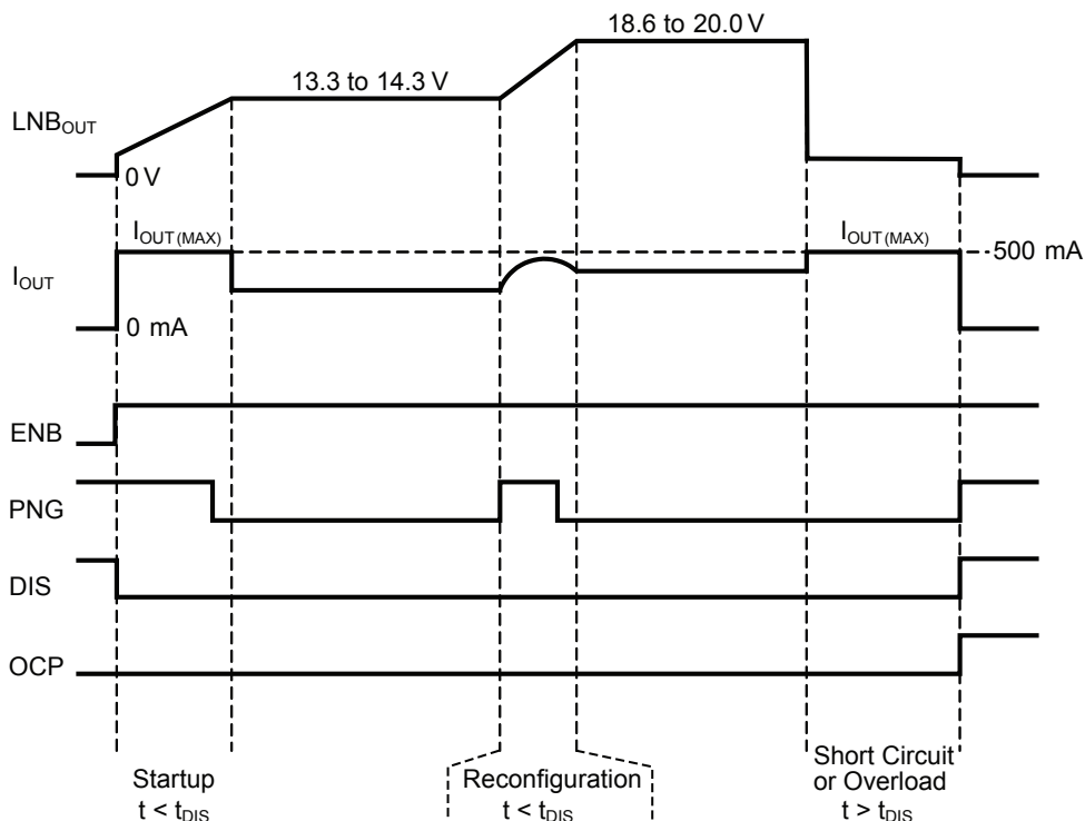
Figure 1. Startup, Reconfiguration, and Short Circuit operation using R_{SET} = 60.4 \text{ k}\Omega , and a capacitive load.
