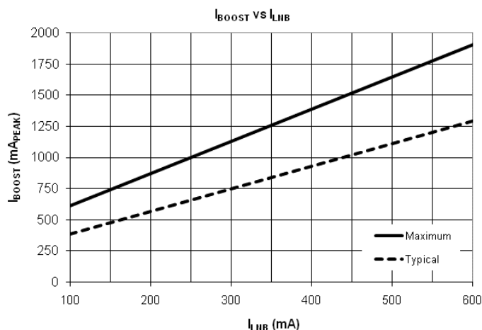
Figure 3. Boost inductor characteristic for the A8296.
