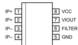
Package LC, 8-Pin SOICN Pinout Diagram
