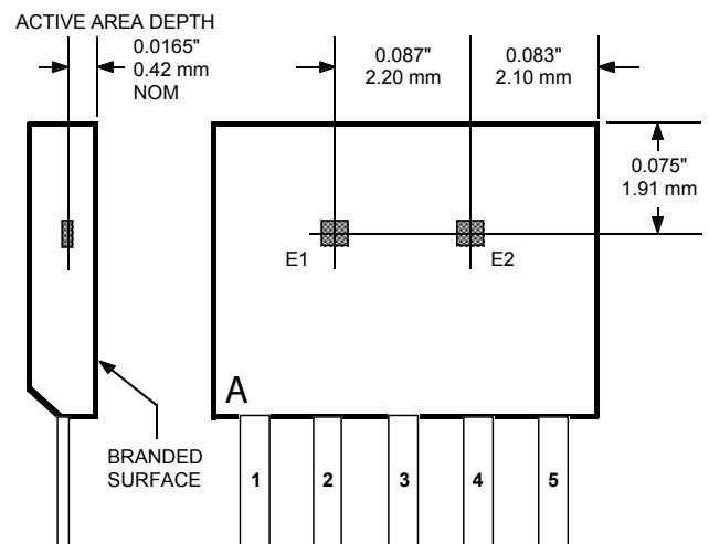
Figure 5 ELEMENT LOCATIONS ( \pm 0.005" [0.13 mm] die placement)
