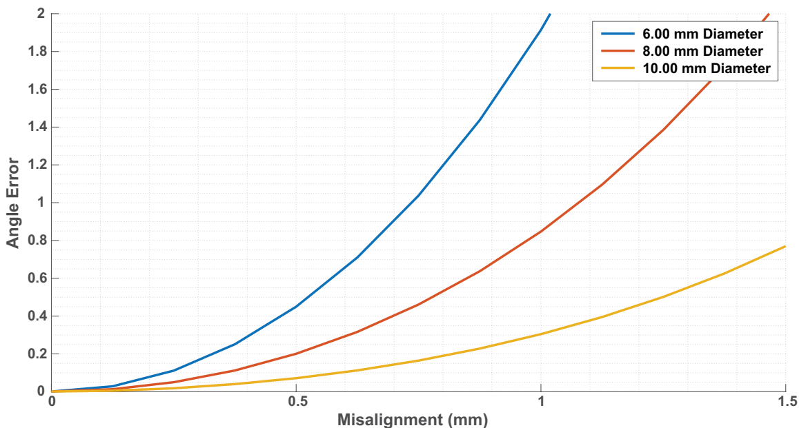
Figure 65: Simulated Error versus Eccentricity for Different Sizes of Magnet Diameters, at 2.0 mm Air Gap
