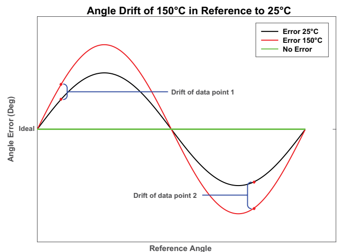
Figure 70: Angle Drift of 150°C in Reference to 25°C [1]
