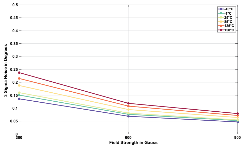
Figure 14: Average 3-Sigma Angle Noise over Field
