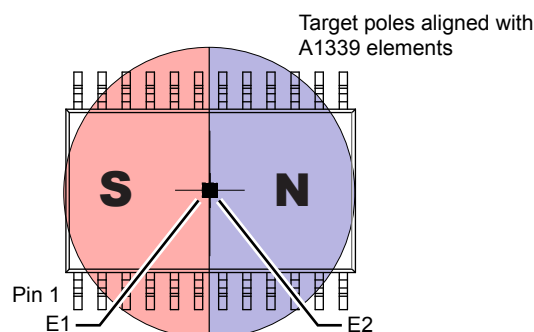
Figure 63: Orientation of Magnet Relative to Primary and Secondary Die
