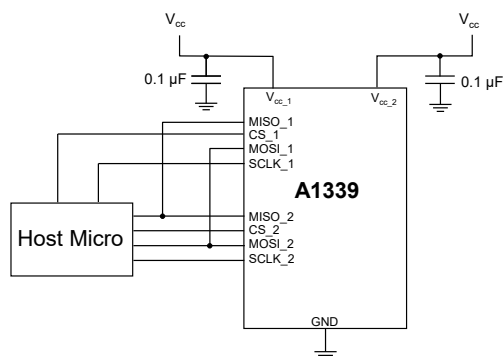
Figure 71: Separate SCLK Lines
