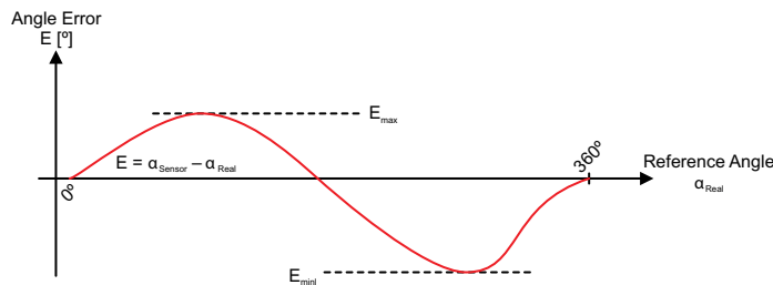
Figure 69: Angle Error Definition
