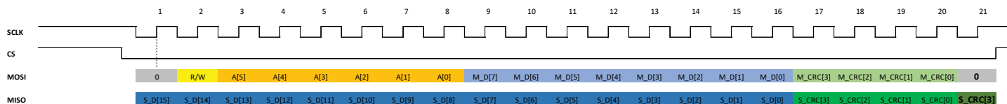
Figure 72: 21-Bit SPI Packet Format
