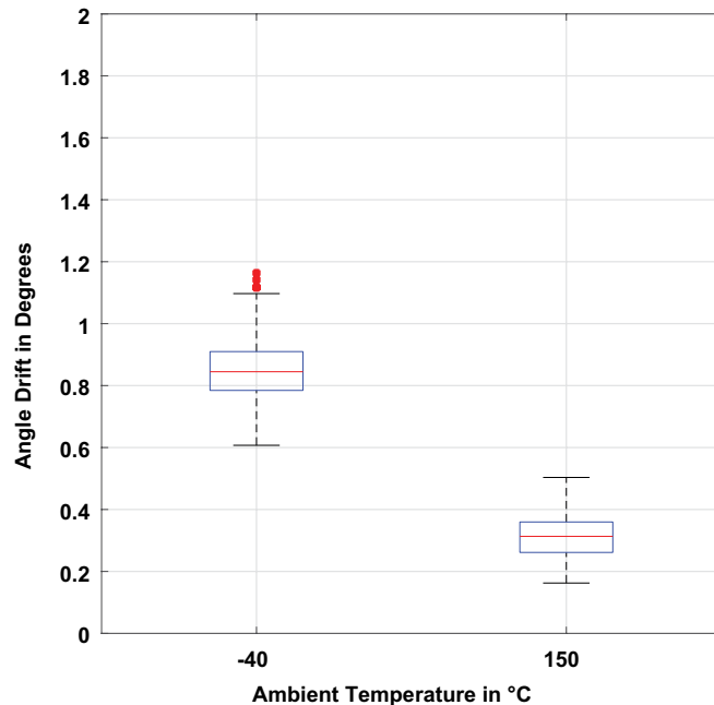
Figure 4: Maximum Absolute Drift from 25°C Reading [1] (300 G)
