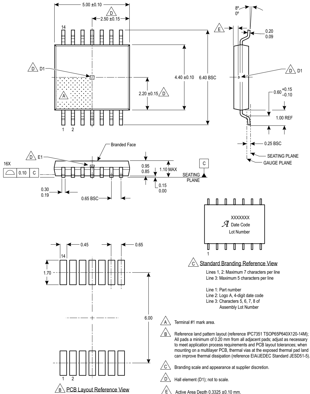
Figure 68: Package LE, 14-Pin TSSOP
