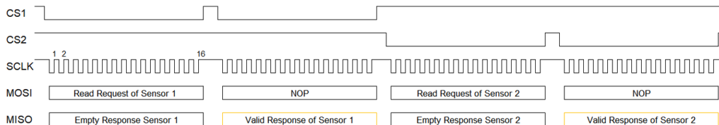
Figure 74: Implementation of SPI Using 16- or 17-Bit Packets; Valid Data, IER Flag Still Asserts
