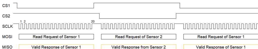
Figure 75: SPI Implementation Using 20-Bit Packets; Data Contents Are Valid; However, IER Flag May Still Assert
