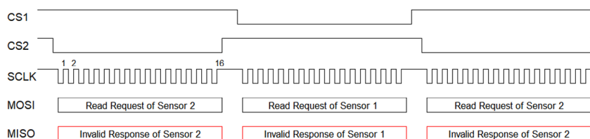
Figure 73: Implementation of SPI Using 16- or 17-Bit Packets Resulting in IER Flag Assertion and Potentially Corrupted Data
