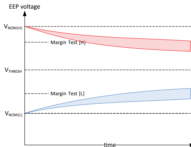
Figure 60: Example of Passing Programming Voltages
