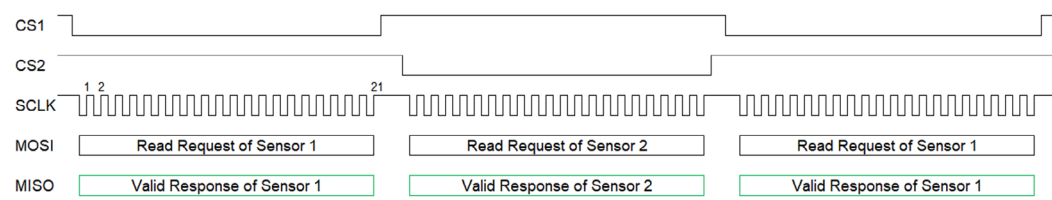
Figure 76: SPI Implementation Using 21-Bit Packets; Data Contents are Valid; No False IER Flag Generation
