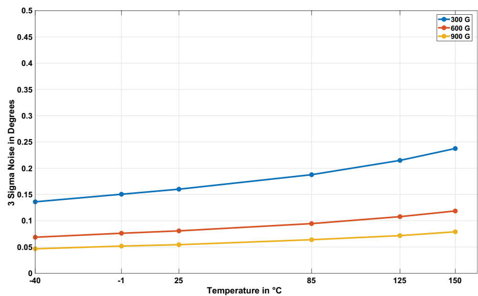
Figure 13: Average 3-Sigma Angle Noise over Temperature
