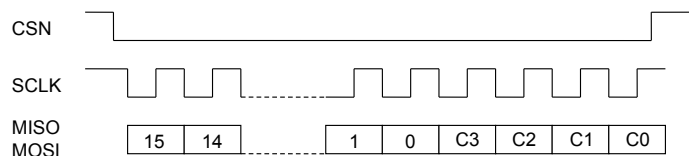
Figure 48: 21-Bit SPI Transaction
