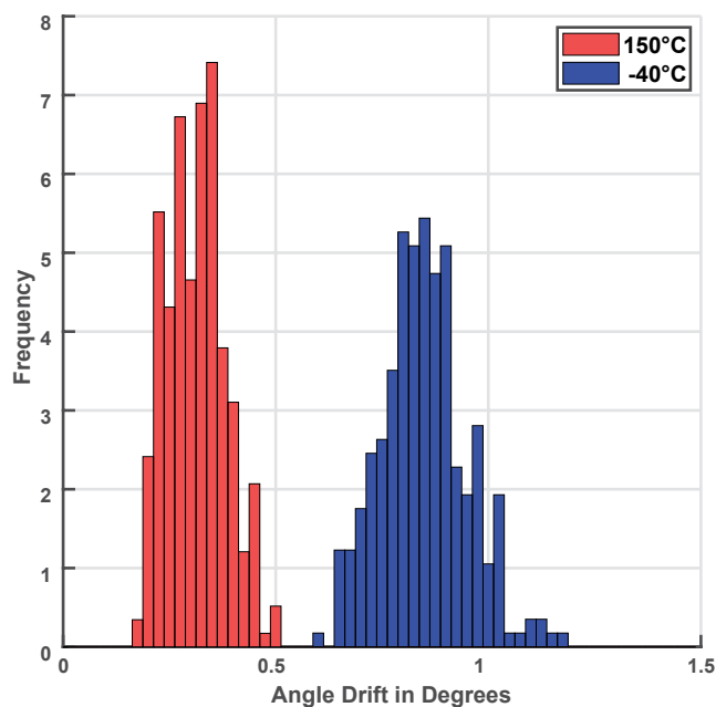
Figure 6: Angle Drift from 25°C (300 G)
