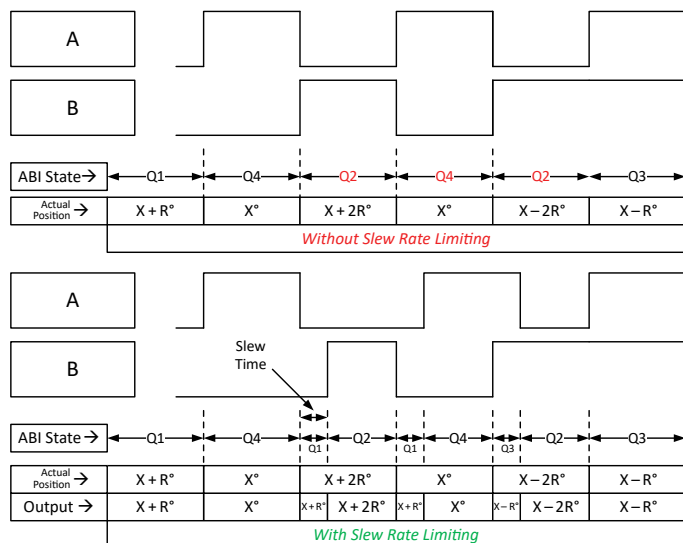
Figure 30: Slew-Rate Limiting
