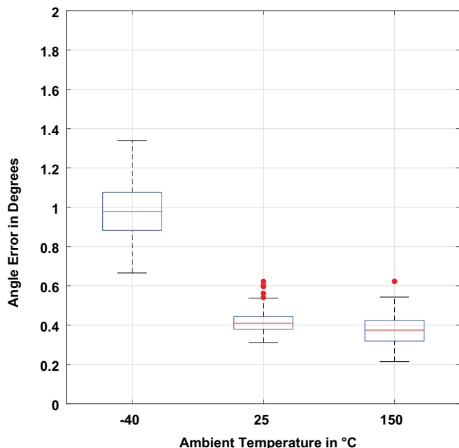
Figure 3: Peak Angle Error over Temperature [1] (300 G)
