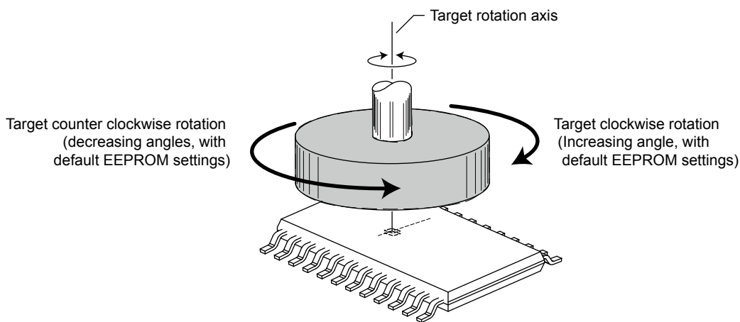
Figure 66: Rotation Direction Definition
