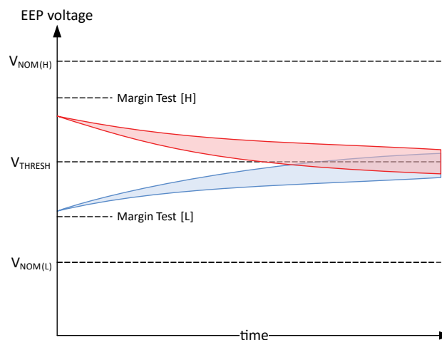
Figure 61: Example of Failing Programming Voltages
